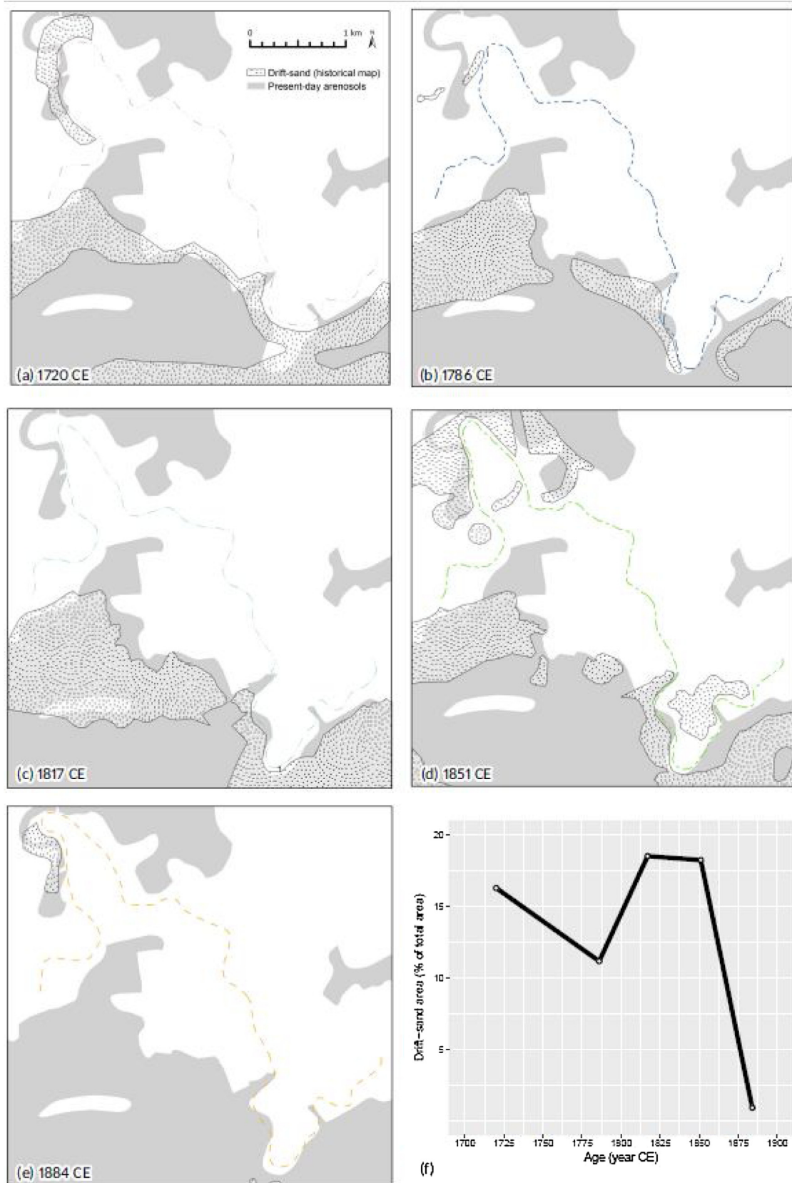
Fig. 5. Development of river planform and drift-sand areas as derived from five historical maps. The dates mentioned are based on the revision date or, if none is given, on the survey date (see Table 2). For the map sheet of the Hottinger atlas the survey covered 3 years; we indicated the middle year in (b). Low-water channel centrelines were derived from the analysis by Quik and Wallinga (2018a). Dotted areas in (a–e) indicate the area covered by drift-sand as displayed on historical maps. Grey shading indicates the area currently classified as arenosols in the Dutch soil classification ('duinvaaggronden' and 'vlakvaaggronden' combined). The graph in (f) shows the relative area covered by drift-sand through time. Source Dutch soil map: Alterra (2014).
