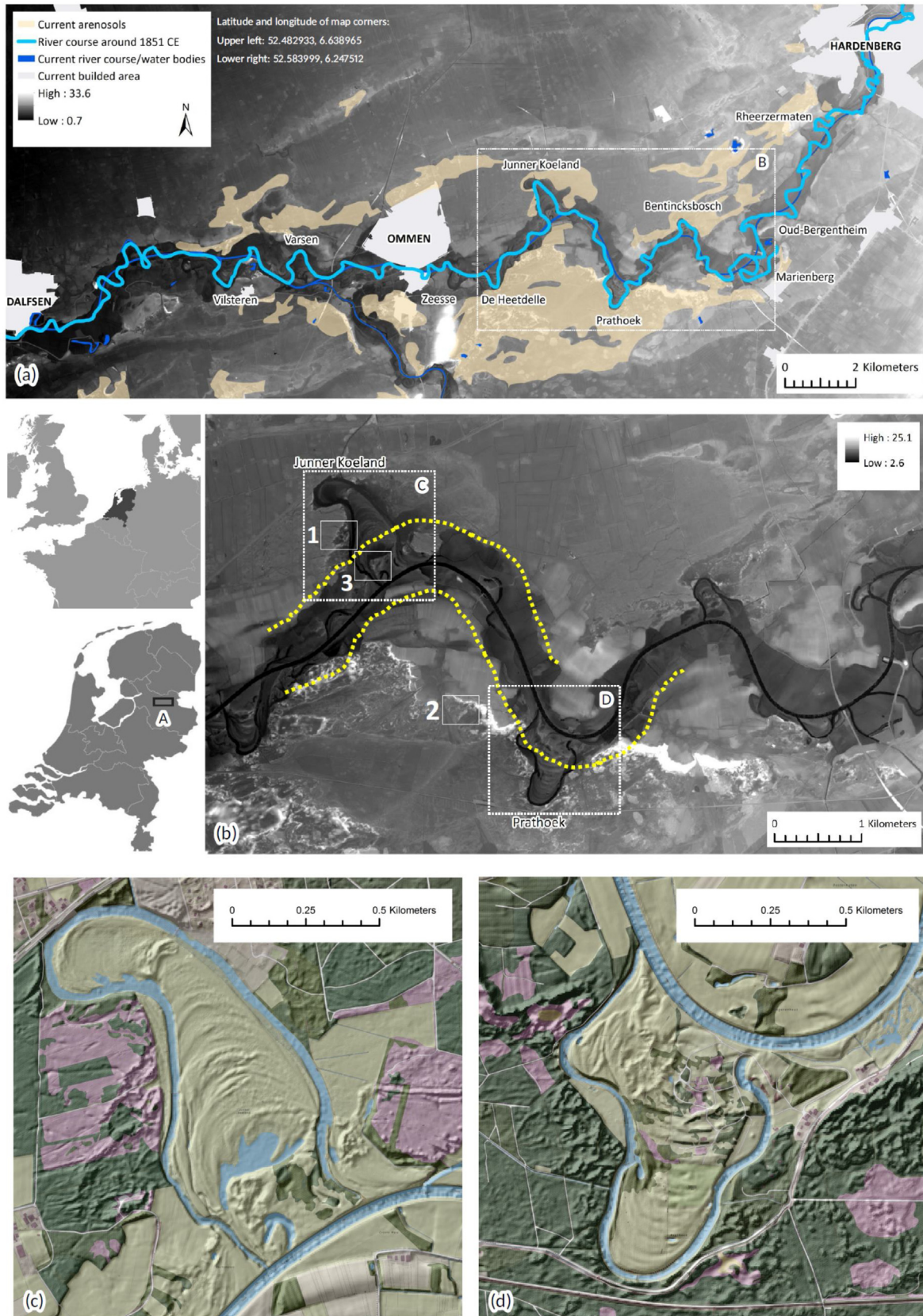
Fig. 1. The Overijsselse Vecht river in the Netherlands. Capitals A–D indicate position of subfigures (a)–(d). (a) Digital elevation model (DEM) of the river reach from Dalfsen to Hardenberg, showing present-day spatial distribution of arenosols (former drift-sand areas, most are currently forested). Meander names are indicated, city names are written in capitals. (b) DEM of the study area showing the two meander bends (Junner Koeland and Prathoek) and the three drift-sand locations (1, 2, 3). Elevation is in meters relative to Dutch Ordinance Datum (roughly mean sea level). The dashed yellow line indicates the valley side, reconstructed at places where large
