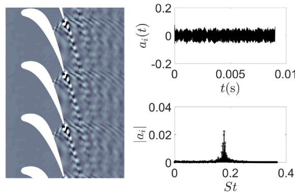
Fig. 14. First POD mode of the temperature fluctuation field T' ; baseline case T_1 = 303.15 K.
