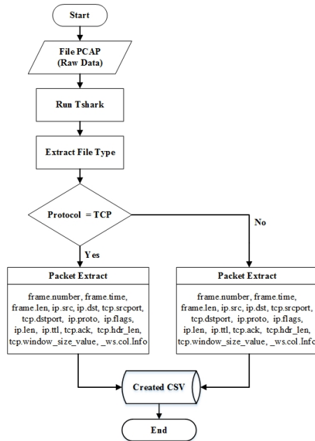
Fig. 3. Flowchart for feature extraction
