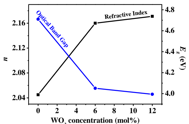
Fig 4. Dependence of Refractive index on WO 3 Concentration.
