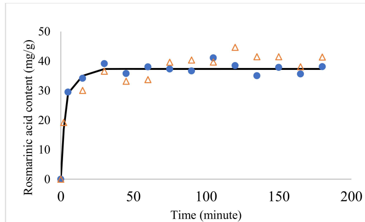
Figure 2. Kinetic profile of rosmarinic acid extraction in preparative- (●) and pilot-scale processes (△) plotted with the predicted first-order kinetic model (line).
