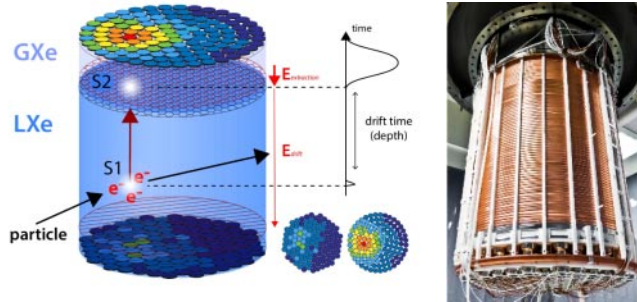
Fig. 1. – Working principle (left) and picture of the XENON1T TPC (right).
