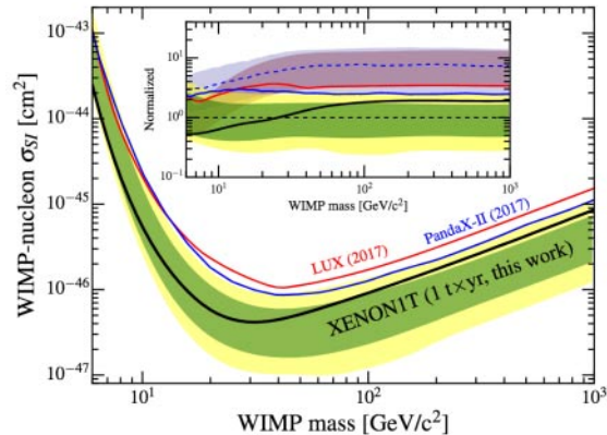
Fig. 3. – Obtained 90% confidence level upper limit on \sigma_{SI} (thick black line) with the 1 \sigma (green) and 2 \sigma (yellow) sensitivity bands. Results from LUX and PandaX-II are shown for comparison. The inset shows these limits and corresponding \pm 1 \sigma bands normalized to the median of this work’s sensitivity band. The normalized median of the PandaX-II sensitivity band is shown as a dotted line.
