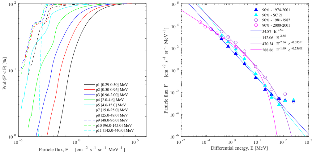
Fig. 1. – (Left) CDFs computed by using proton flux data in the energy channels (P1-P11) of the IMP-8/CPME instrument. (Right) Proton flux spectra (symbols) obtained from IMP-8/CPME and their fits (lines) over the total acquisition time (January 1974 - October 2001, blue), the SC No. 21 (cyan) and its maximum phase (1981-1982, purple). Proton flux spectrum obtained from EPAM/LEMS120 aboard ACE and its fit over the maximum phase of solar cycle No. 23 (2000-2001, pink circles and pink line, respectively).
