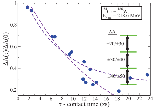
Fig. 3. – The ratio of the final and initial fragment masses as a function of contact time for the ^{54}\text{Cr} + ^{186}\text{W} system at E_{\text{c.m.}} = 218.6 \text{ MeV} and for two orientations of the ^{186}\text{W} nucleus. Dashed lines show two possible fits.
