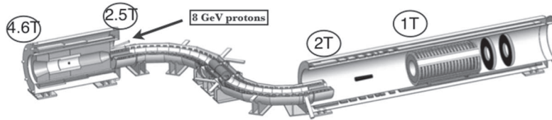
Fig. 1. – Experimental layout of Mu2e. The Cosmic ray veto is not shown.
