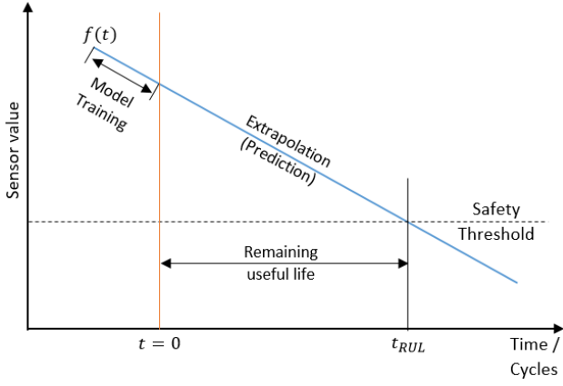
Fig. 6. The evaluation remaining useful life by regressive event tracking model.
