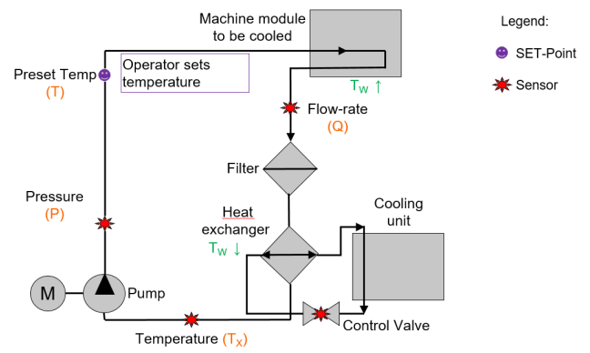
Fig. 2. Schematic of thermal regulator of continuous compression machine.
