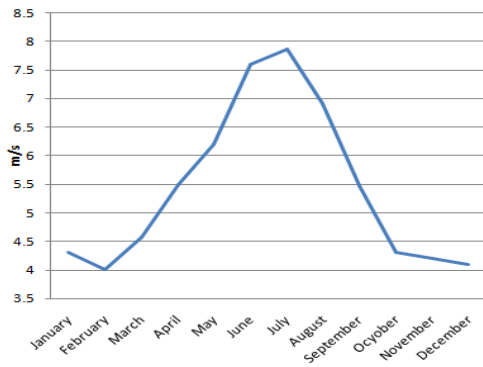
Fig. 2 Graph of Monthly average daily Wind Speed in Sandwip [5]
