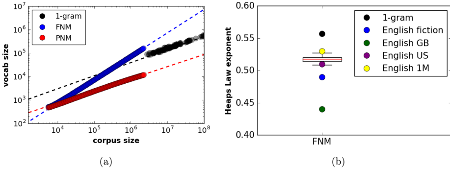
Fig. 3. (Color online) Heaps law in simulated Neutral models versus 1-gram data. (a) A double-logarithmic plot, showing corpus size versus vocabulary size, i.e., Heaps Law, for all 1-grams (black), the FNM (blue) and the PNM (red). (b) The Heaps law exponents, \beta , for the data series on the left, as well as additional data series, using Table 1 in [40]: all English 1-grams: 0.54 \pm 0.01 ; English fiction: 0.49 \pm 0.01 ; English GB: 0.44 \pm 0.01 ; English US: 0.51 \pm 0.01 . The 100 independent runs of each neutral model, using parameters listed in the text, yielded \beta = 0.52 \pm 0.07 for the PNM, and \beta = 1.00 \pm 0.002 for the FNM (not shown).
