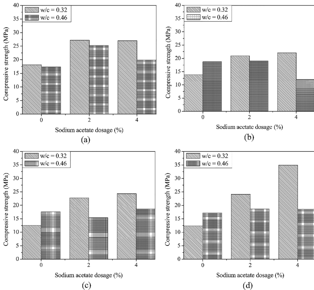
Fig. 7. Compressive strength of concrete after: (a) curing under -25\text{ }^{\circ}\text{C} for 7 days, (b) curing under -25\text{ }^{\circ}\text{C} for 28 days, (c) curing under 60\text{ }^{\circ}\text{C} for 7 days and (d) curing under 60\text{ }^{\circ}\text{C} for 28 days.
