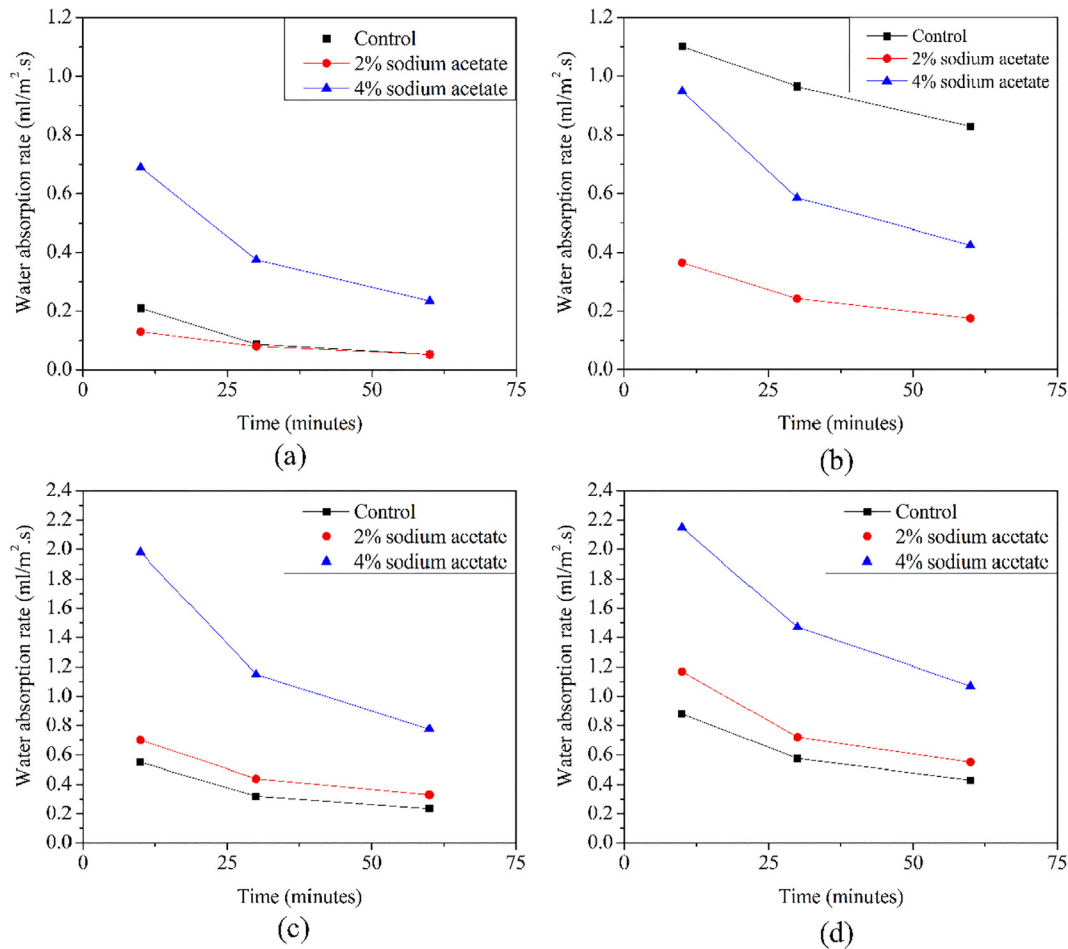
Fig. 6. Water absorption rate at 28 days for concrete with (a) w/c = 0.32 cured under -25^{\circ}\text{C} , (b) w/c = 0.32 cured under 60^{\circ}\text{C} , (c) w/c = 0.46 cured under -25^{\circ}\text{C} and (d) w/c = 0.46 cured under 60^{\circ}\text{C} .
