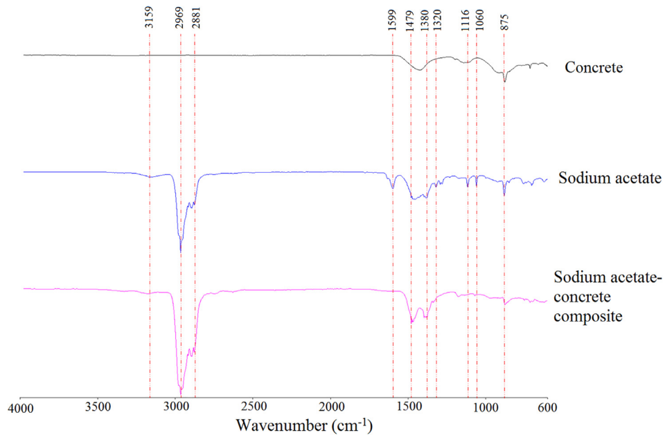
Fig. 4. FTIR analysis of sodium acetate and concrete [16].
