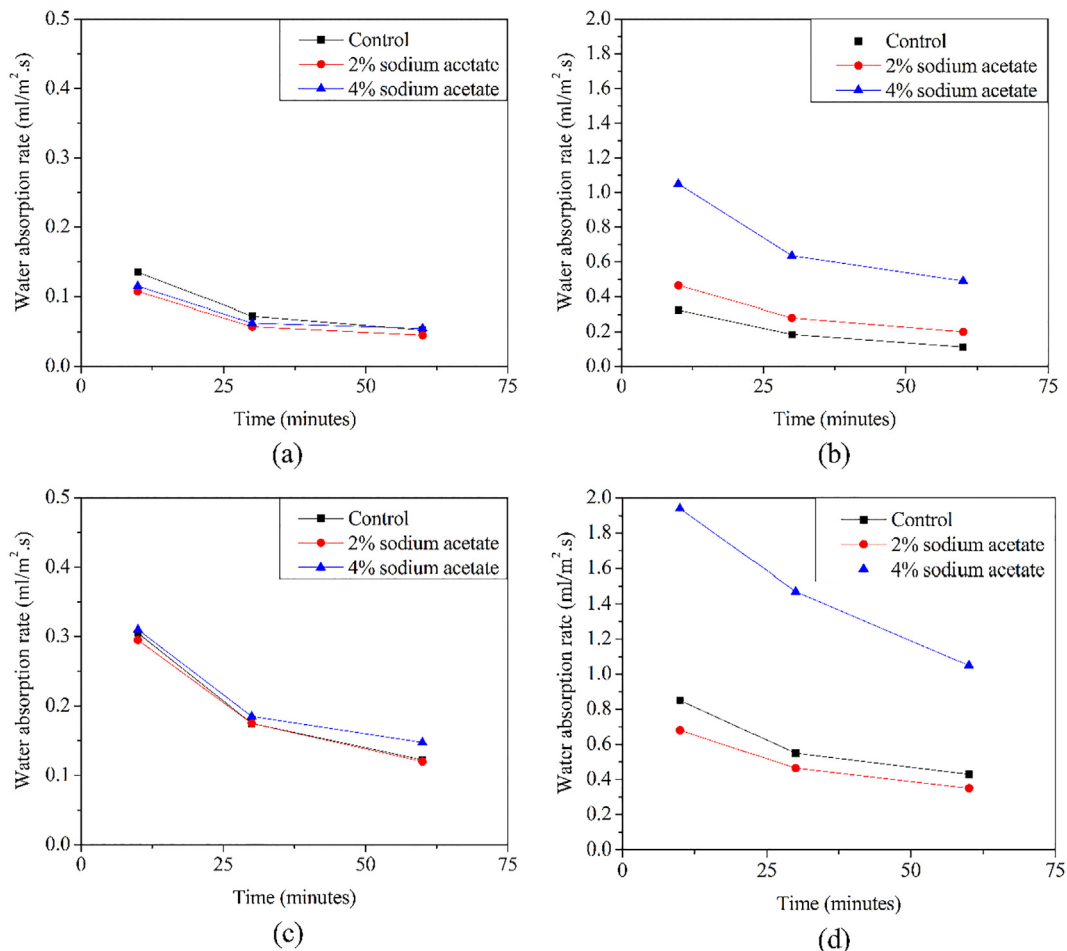
Fig. 5. Water absorption rate at 7 days for concrete with (a) w/c = 0.32 cured under -25^\circ\text{C} , (b) w/c = 0.32 cured under 60^\circ\text{C} , (c) w/c = 0.46 cured under -25^\circ\text{C} and (d) w/c = 0.46 cured under 60^\circ\text{C} .
