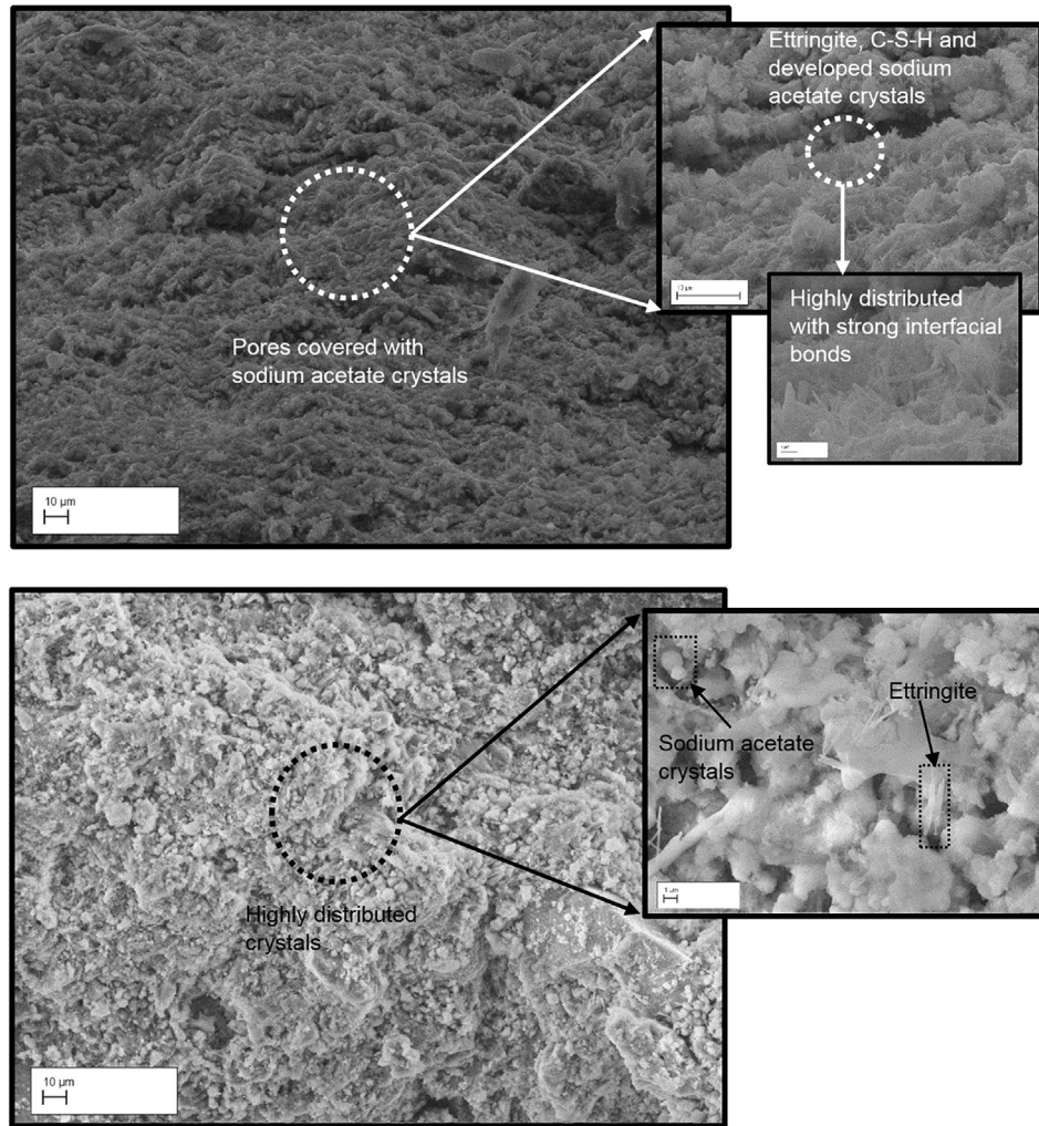
Fig. 3. Morphology of concrete incorporated with sodium acetate and cured under extreme conditions of: (a) -25\text{ }^{\circ}\text{C} (1000 \times , 5000 \times and 20,000 \times ) and (b) 60\text{ }^{\circ}\text{C} (1000 \times , 5000 \times and 20,000 \times ).
