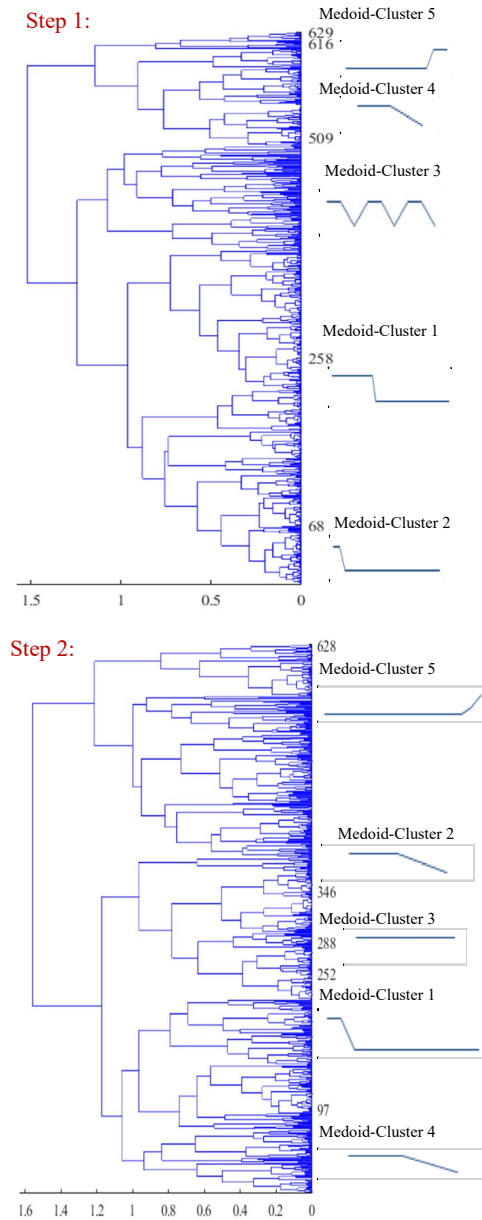
Fig. 3. Temporal phenotypes (The First Hidden Clusters ‘Profiles’) in hierarchical clustering. Deprograms of Hierarchical clustering (complete) for the first and second hidden variable with the DTW distance metric. The x-axis represents a measure of closeness of either individual data points or clusters, while y-axis is representing patient IDs as data points.
