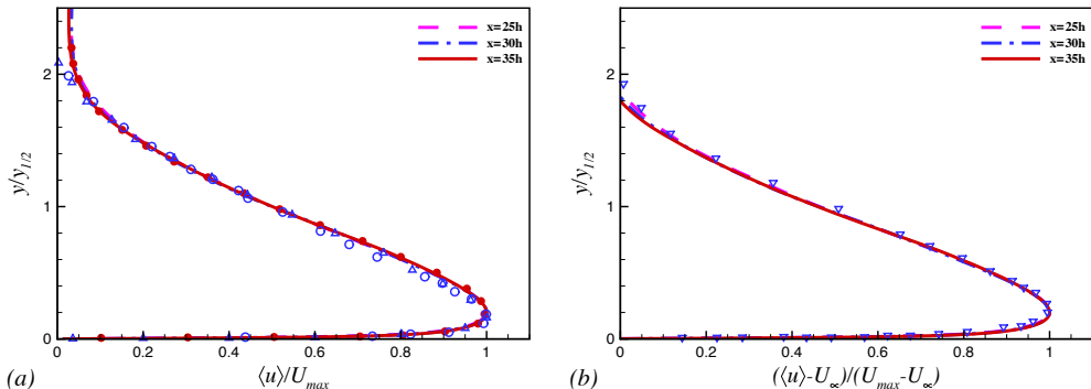
Figure 11: Mean streamwise velocity profiles scaled with outer length scales (a) \langle u \rangle / U_{max} and (b) (\langle u \rangle - U_{\infty}) / (U_{max} - U_{\infty}) . LES of Banyassady & Piomelli (2014) ( \bullet ), x = 30h . Experimental data: Rostamy et al. (2011a) ( \circ ), x = 30h ; Eriksson et al. (1998) ( \triangle ), x = 40h ; Irwin (1973) ( \nabla ), x = 82.2h .
