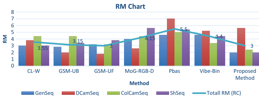
Figure 10. RM chart shows the overall performance of CLW , GSM_{UF} , GSM_{UB} , MoG_{RGB-D} .PBAS and ViB_{bin} and proposed method in GenseqSeq, DCamSeq, ColCamSeq and Shseq sequences. The lower then RM and RC values are the better the performance is.
