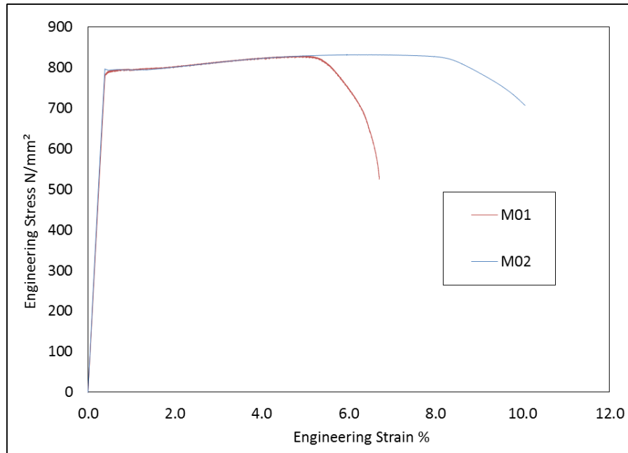
Figure 8: Effect of specimen geometry on S690 at quasi-static loading condition. Courtesy of TWI Ltd.
