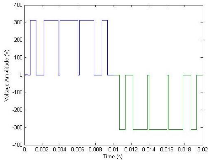
Figure 3: Voltage output for m_f=5 . The modulation index is M=0.9837 and the voltage amplitude of the fundamental is U_{(1)}=217,29 \text{ V} .
