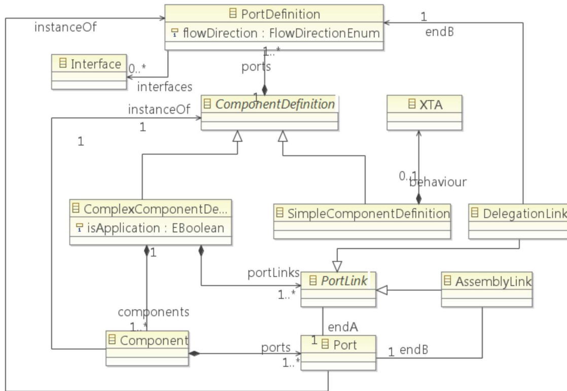
Figure 1: Excerpt of WCOMM metamodel
