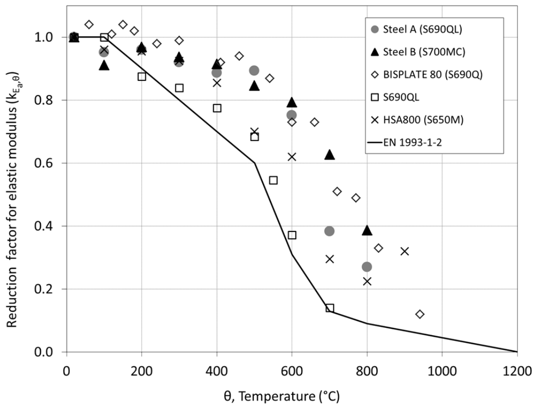
Figure 11: Reduction factors for the elastic modulus
