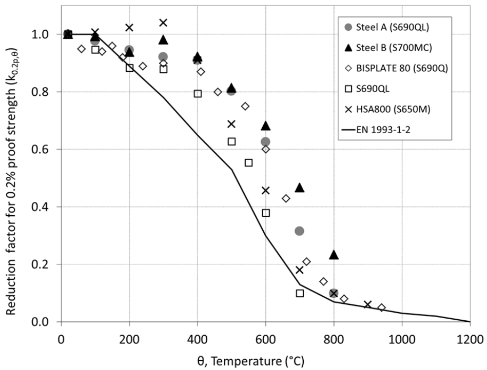
Figure 9: Reduction factors for the 0.2% proof strength
