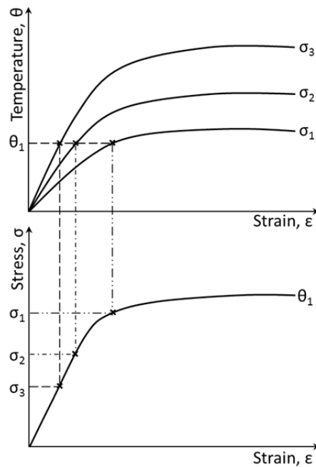
Figure 4: Converting temperature-strain curves from transient test result into stress-strain curves
