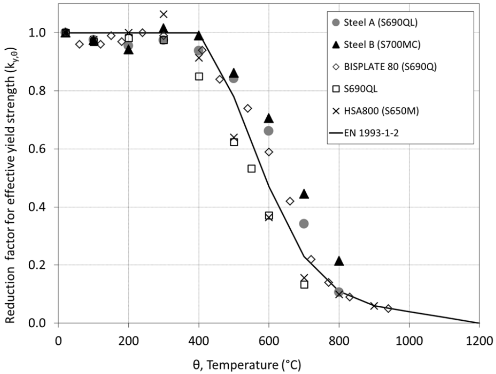
Figure 10: Reduction factors for the 2% yield strength
