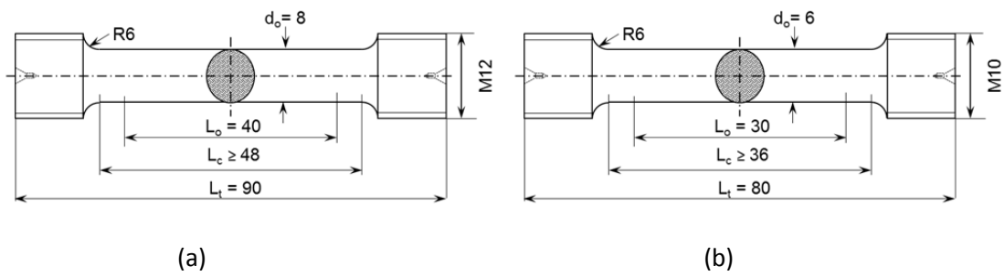
Figure 2: Dimensions of a (a) M12 and (b) M10 tensile specimen (all measurements are in mm)
