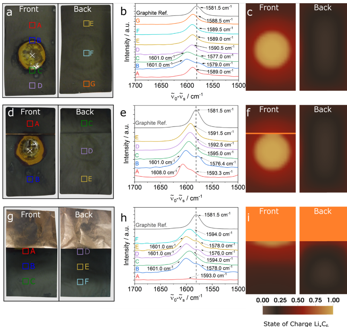
Figure 8. Experiments with typical electrolyte solution with conductive salt. (a)–(c) Unmodified graphite electrode. (a) The squares ( 0.25 \text{ cm}^2 ) emphasize the measured positions for Raman spectroscopy in the respective color. The white X marks the former center of the Li-metal disk. (b) Raman spectra of electrode after 4 weeks at 29^\circ \text{C} and pristine graphite electrode as reference. (c) State of Charge distribution calculated with the simulation. (d)–(f) Electrode setup with interrupted electrode coating after 4 weeks at 29^\circ \text{C} . (d) Squares ( 0.25 \text{ cm}^2 ) show in which zones Raman spectroscopy was conducted. The white X marks the former center of the Li-metal disk. (e) Raman spectra of the sample and pristine graphite electrode as reference. (f) SOC distribution calculated with the simulation. (g)–(i) Electrode setup with Li in contact with the Cu foil after 4 weeks at 29^\circ \text{C} . (g) Squares ( 0.25 \text{ cm}^2 ) show in which zones Raman spectroscopy was conducted. (h) Raman spectra of the sample and pristine graphite electrode as reference. (i) SOC distribution of the simulation.
