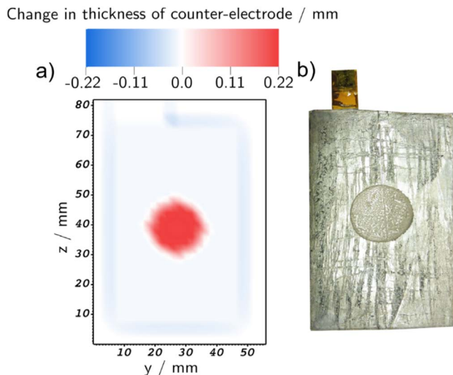
Figure 4. (a) Thickness variation on the surface of the counter-electrode at the end of the simulation. (b) Image of Li counter electrode after cell opening.
