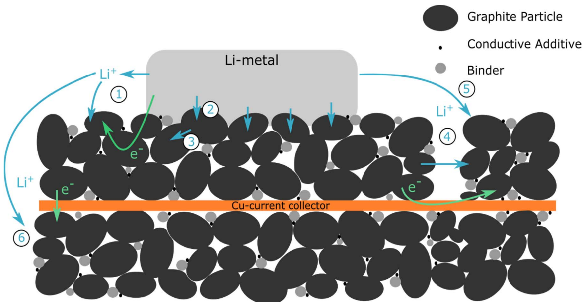
Figure 5. Possible Li transport pathways in the reaction of Li metal with a graphite electrode.
