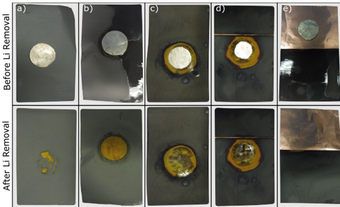
Figure 6. Overview of all setups after 4 weeks at 29 °C. (a) Without electrolyte. (b) With EC:EMC (3:7) + 2wt.% VC. (c) 1 M LiPF 6 in EC:EMC (3:7) + 2wt.% VC. (d) Interrupted electrode (1 mm) in 1 M LiPF 6 in EC:EMC (3:7) + 2wt.% VC. (e) Li pressed on copper in 1 M LiPF 6 in EC:EMC (3:7) + 2wt.% VC.
