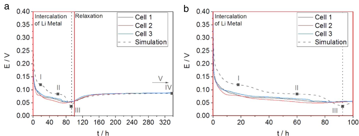
Figure 2. (a) Cell voltage of the three measured cells and the electrochemical simulation. Four of the five points for selected 3D results in Fig. 3 are marked with squares. A voltage minimum is reached between 74 h–84 h (experiment) and 92 h (simulation). The red square emphasizes the zoomed in part for (b).
