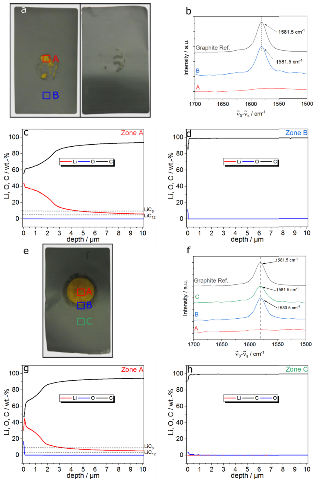
Figure 7. (a)–(d) Example for the characterization of the lithiation state of the electrodes after 4 weeks in case of the setup without electrolyte. (a) Squares ( 0.25 \text{ cm}^2 ) show in which zones Raman spectroscopy and GD-OES were conducted. (b) Raman spectra of the sample. Upper spectrum from pristine graphite electrode. (c) GD-OES depth profiling of zone A. (d) GD-OES depth profiling of zone B. (e)–(h) Electrode setup with carbonate solution without \text{LiPF}_6 after 4 weeks at 29^\circ \text{C} . (e) Squares ( 0.25 \text{ cm}^2 ) show in which zones Raman spectroscopy and GD-OES were conducted. (f) Raman spectra of the sample. Upper spectrum from pristine graphite electrode. (g) GD-OES depth profiling of zone A. (h) GD-OES depth profiling of zone C.
