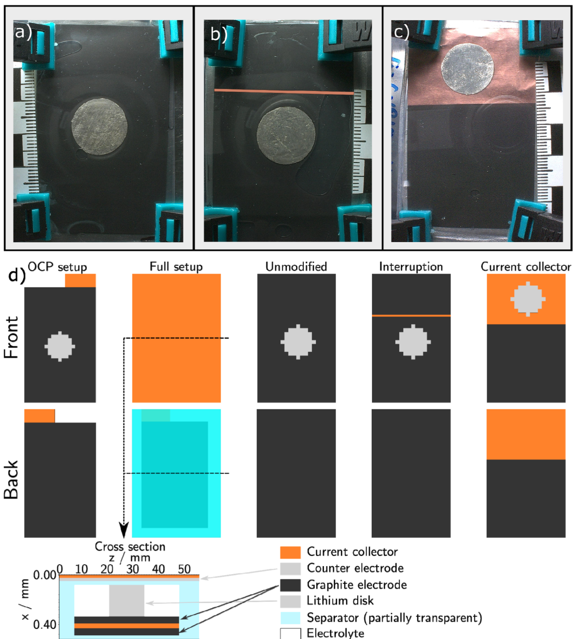
Figure 1. Experimental setups with Li metal disk on graphite electrode (a) unmodified, (b) with 1 mm interruption of graphite coating (the position of the interruption was enhanced graphically for better visibility), (c) Li metal disk on Cu current collecting foil, not in direct contact with coating. (d) The simulated electrodes for the four different setups from the front and the back and the full simulation domain with a cross section are shown.
