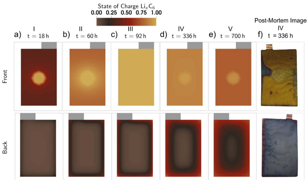
Figure 3. The lithiation state of the front and back graphite electrode from (a)–(e) simulations and (f) experiment.
