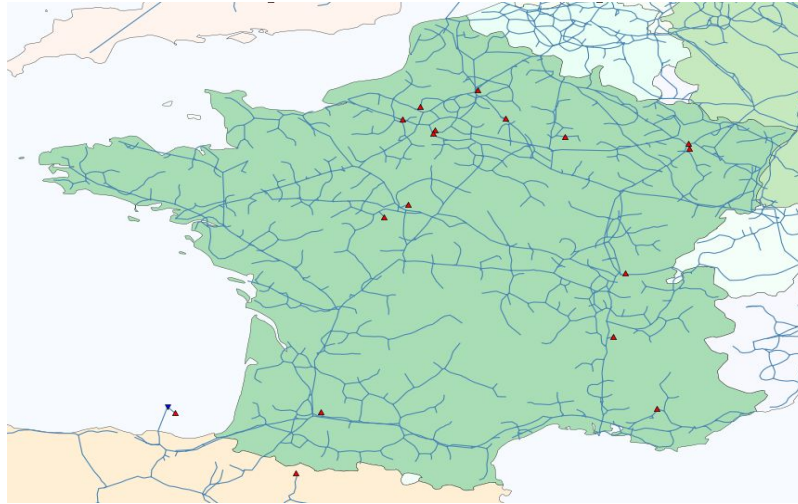
Figure 3.20: SciGRID_gas data set for France.
