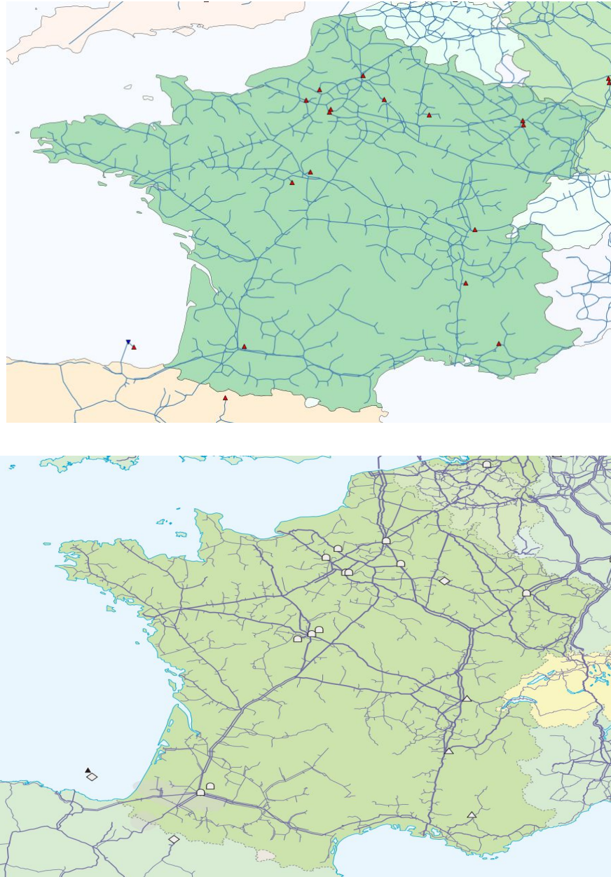
Figure 5.2: SciGRID_gas (top) and EntsoG (bottom) pipelines for France
