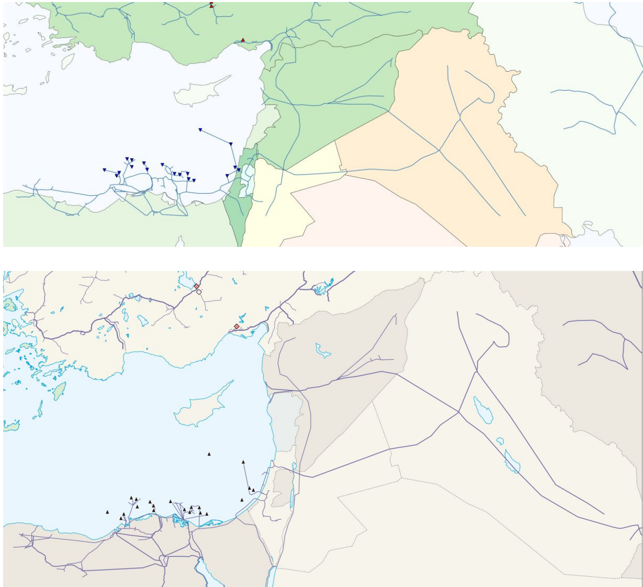
Figure 5.15: SciGRID_gas (top) and EntsoG (bottom) pipelines for East Africa
