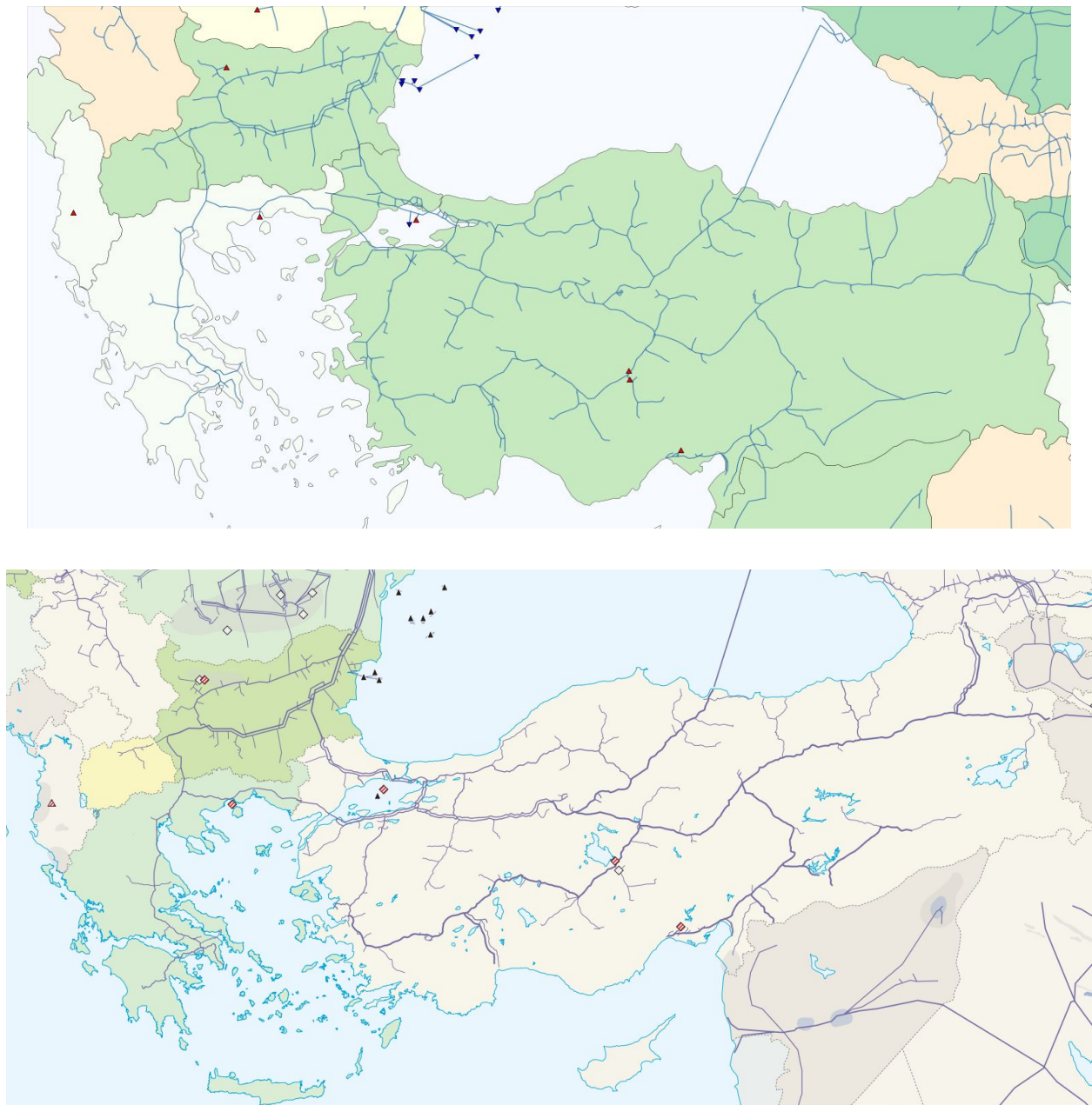
Figure 5.6: SciGRID_gas (top) and EntsoG (bottom) pipelines for Greece, Turkey and Bulgaria
