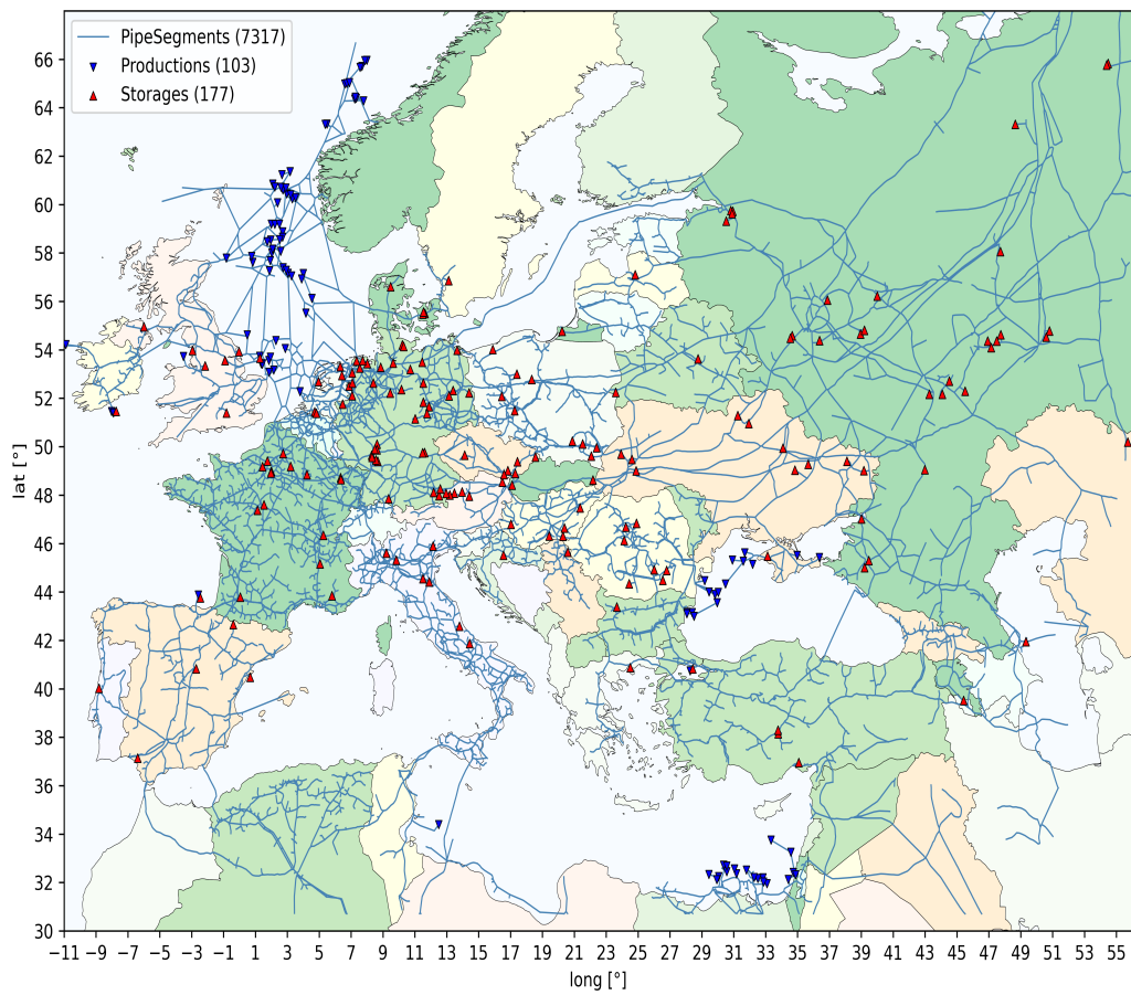
Figure 3.19: The pipelines, storage facilities and production sites of the EMAP data set.
