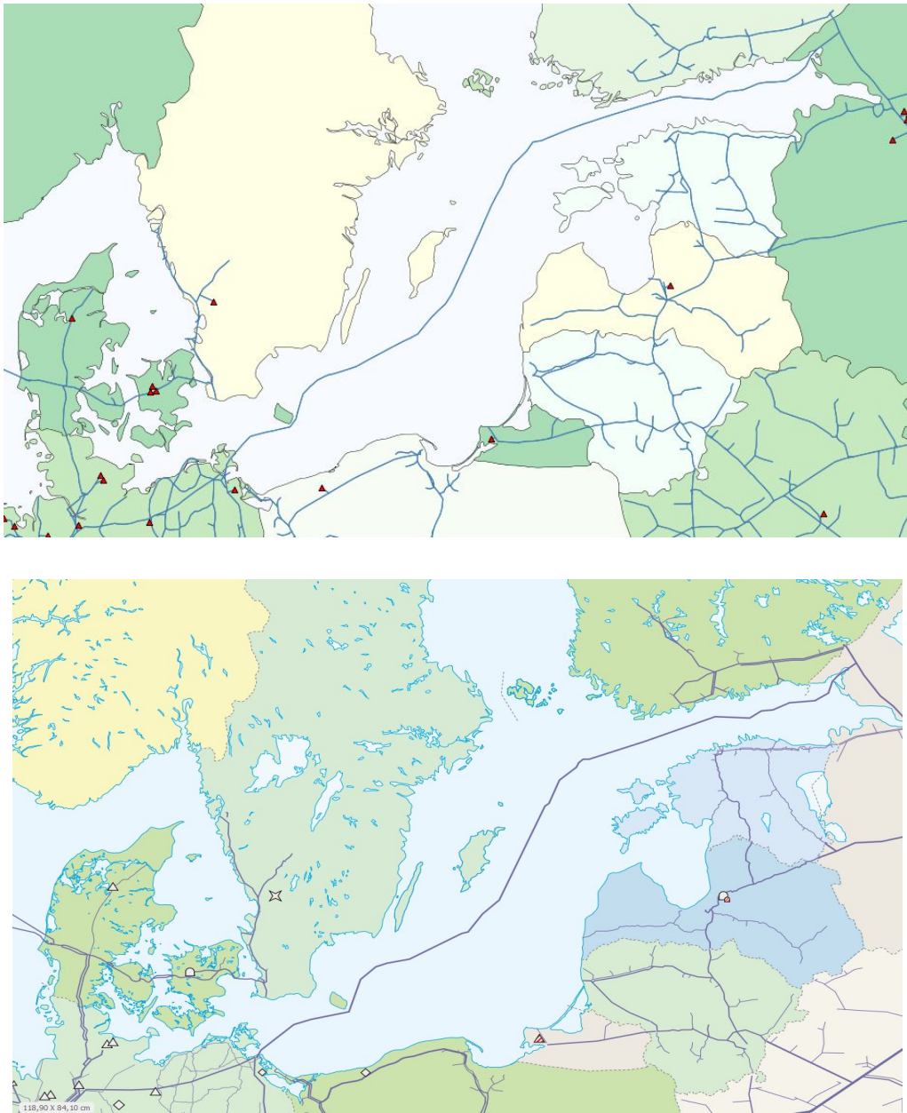
Figure 5.11: SciGRID_gas (top) and EntsoG (bottom) pipelines for the Baltic Sea
