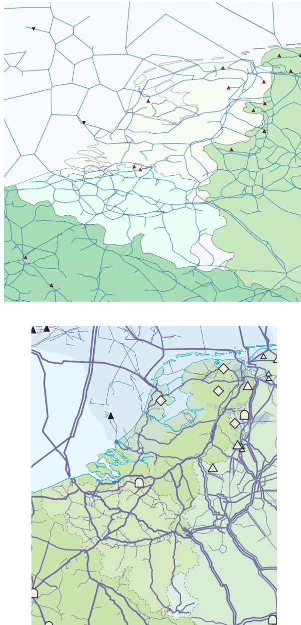
Figure 5.4: SciGRID_gas (top) and EntsoG (bottom) pipelines for Belgium, Holland and Luxembourg
