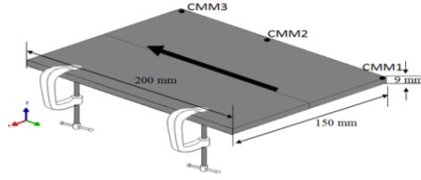
Figure 1: Experimental Setup for 9-mm Low Carbon Steel
