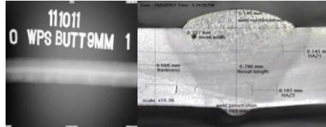
Figure 2: Digital X-ray and Macrograph
