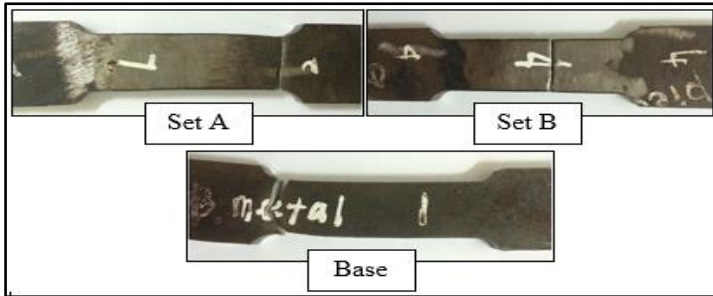
Figure 5: Fatigue Life Fracture on Set A, B and Base specimen.
