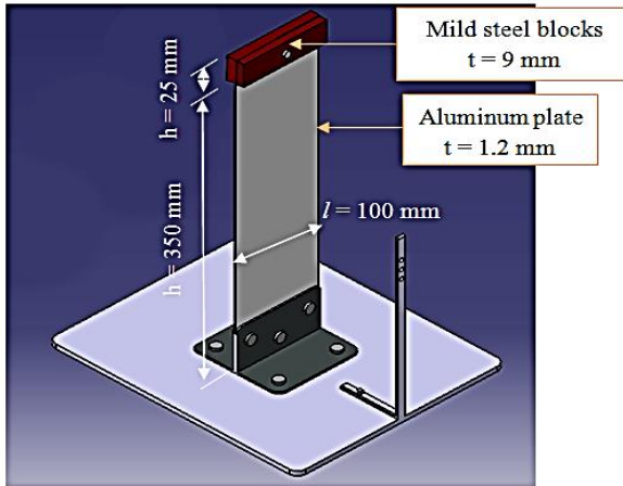
Figure 1: Main system
