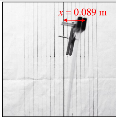
Figure 11(b): DM dynamic absorber in vertical position
