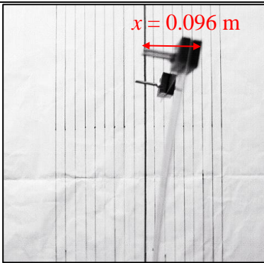
Figure 11(a): DM dynamic absorber in horizontal position
