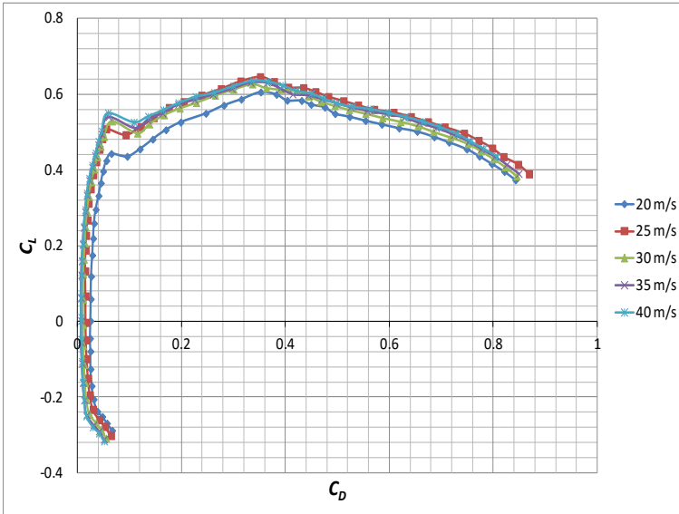
Fig. 11 Lift coefficient ( C_L ) versus drag coefficient ( C_D )
