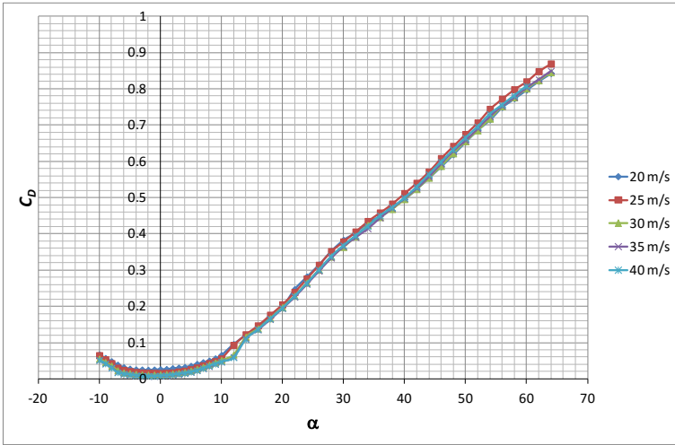
Figure 6: Drag coefficient ( C_D ) versus angle of attack ( \alpha ).
