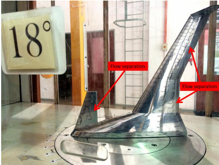
Figure 8: Visualisation at \alpha = 18^\circ
