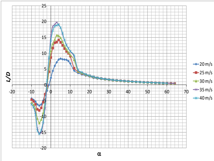
Figure 9: Lift-to-drag ratio (L/D) versus angle of attack ( \alpha )
