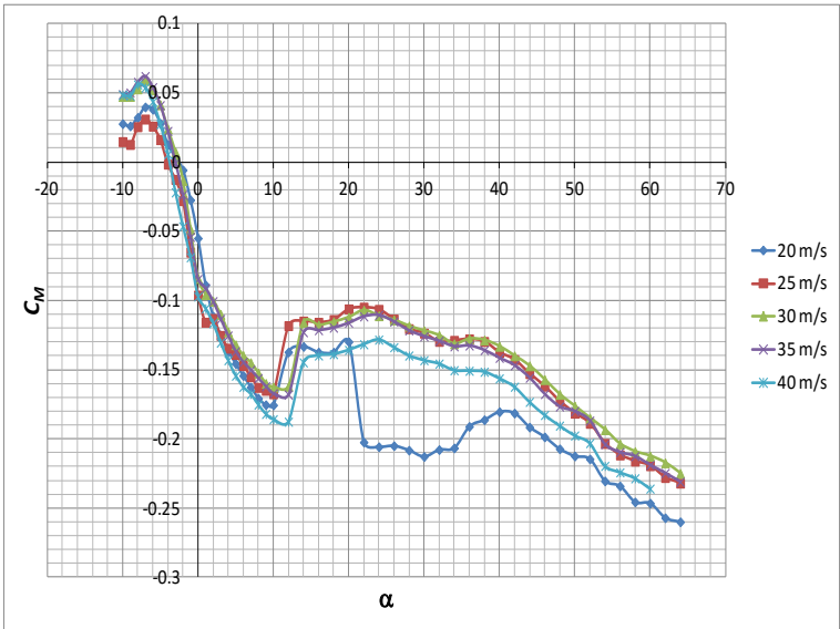
Figure 12: Pitching moment coefficient ( C_M ) versus angle of attack ( \alpha )
