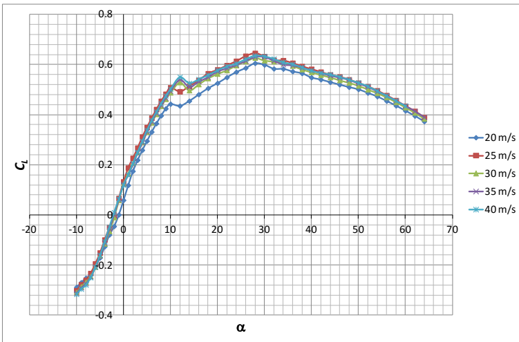
Figure 4: Lift coefficient ( C_L ) versus angle of attack ( \alpha ).
