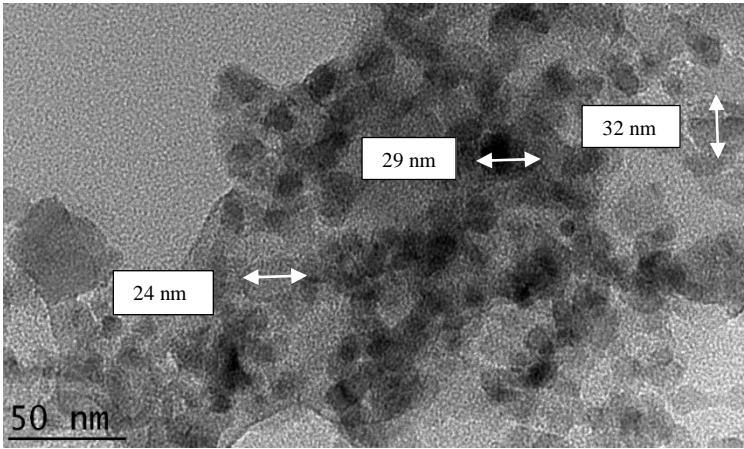
Figure 1 (a): TEM image of \text{SiO}_2/\text{PAG} nanolubricant at X 88,000 magnifications.
