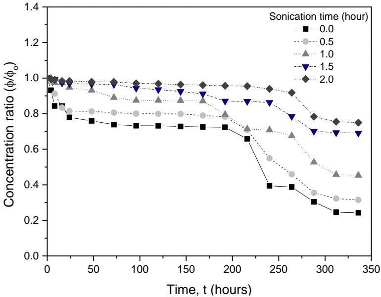
Figure 5: Absorbance ratio of SiO 2 /PAG nanolubricant for different sonication time as a function of time.
