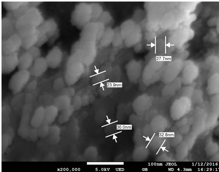
Figure 1(b): FESEM image of \text{SiO}_2 nanoparticle powder at X 200,000 magnifications.
