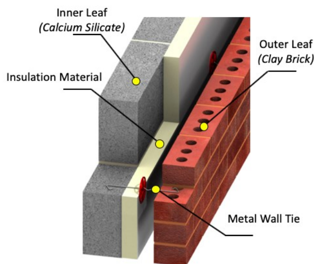
Figure 1. Cavity wall
