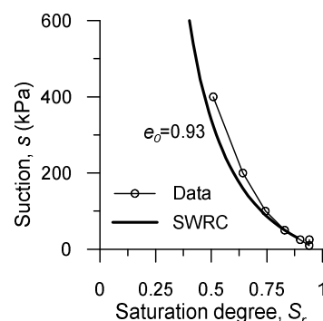
Fig. 1. Soil water retention curve.
