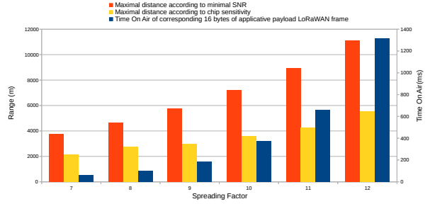
Fig. 2. LoRa TM analytic tradeoffs between TOA and transmission range against spreading factors.
