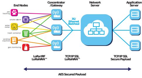
Fig. 1. LoRaWAN networking architecture from [12].
