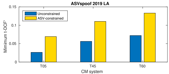
Fig. 5. Comparison of the unconstrained and ASV-constrained minimum t-DCF for the top three systems of the ASVspoof 2019 LA challenge ( \pi_{\text{spoofer}} = 0.05 ). For t-DCF both ASV and CM thresholds are chosen to minimize the cost, while for ASV-constrained t-DCF, the ASV is set to its EER point.
