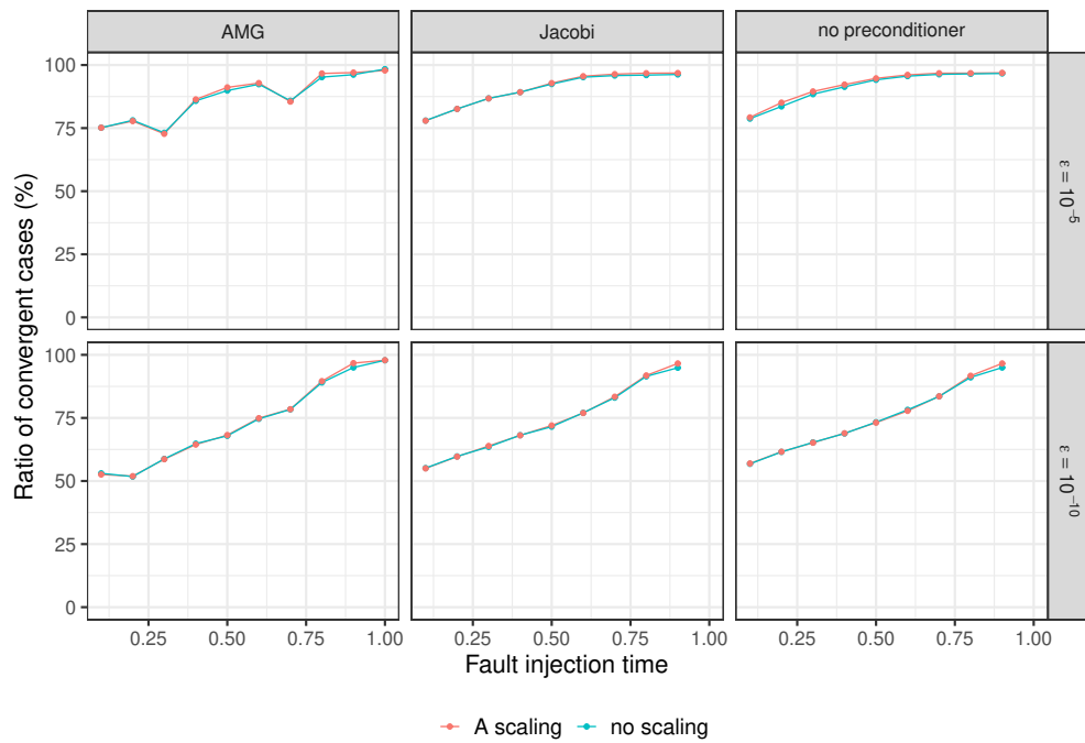
Figure 1.3: Impact of the bit-flip injection time (as a proportion of the number of iterations with respect to the non-faulty execution) in the matrix-vector product on PCG convergence success.
