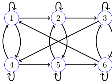
Figure 1: Nonsplit digraph with radius 3. For example, node 1 and 6 have common incoming neighbor 6, while nodes 1 and 5 have node 4 as common incoming neighbor.
