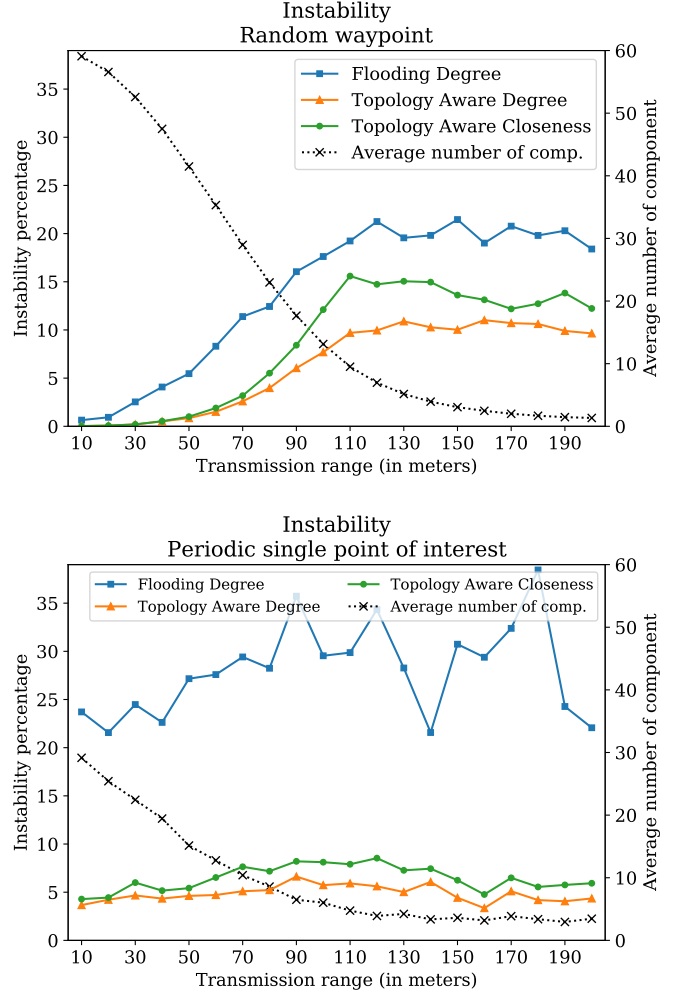
Figure 2. Instability percentage
