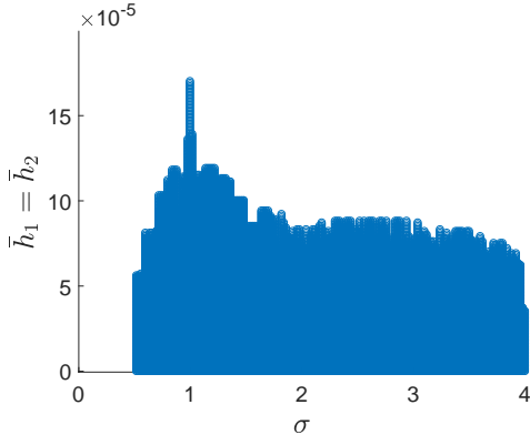
Fig. 2: Trade-off between coupling strength \sigma and maximum sampling interval \bar{h}_1 = \bar{h}_2 , for the system (40), with \alpha = 0.01 .
