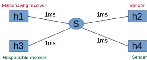
Fig. 4. Experimental topology used in mininet
