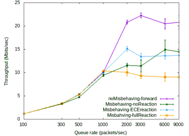
Fig. 6. Responsive h3-h4 flow throughput depending on the output queue rate
