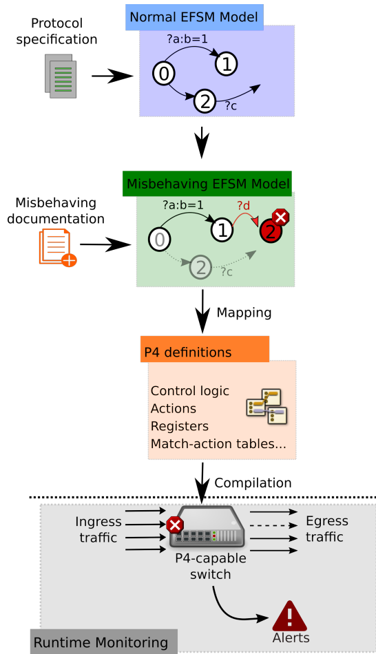
Fig. 1. Approach overview
