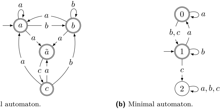
■ Figure 6 Automata corresponding to the specialized DTD a \rightarrow (a + b + \tilde{a})^* , b \rightarrow (a + b + \tilde{a})^* , \tilde{a} \rightarrow c^* , c \rightarrow (a + b)^* with alphabet projection a \mapsto a , \tilde{a} \mapsto a , b \mapsto b , c \mapsto c .
