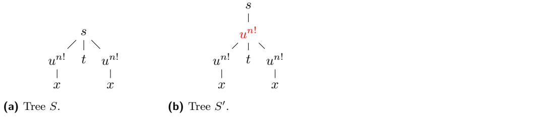
■ Figure 4 Fooling trees in Lemma 25.
