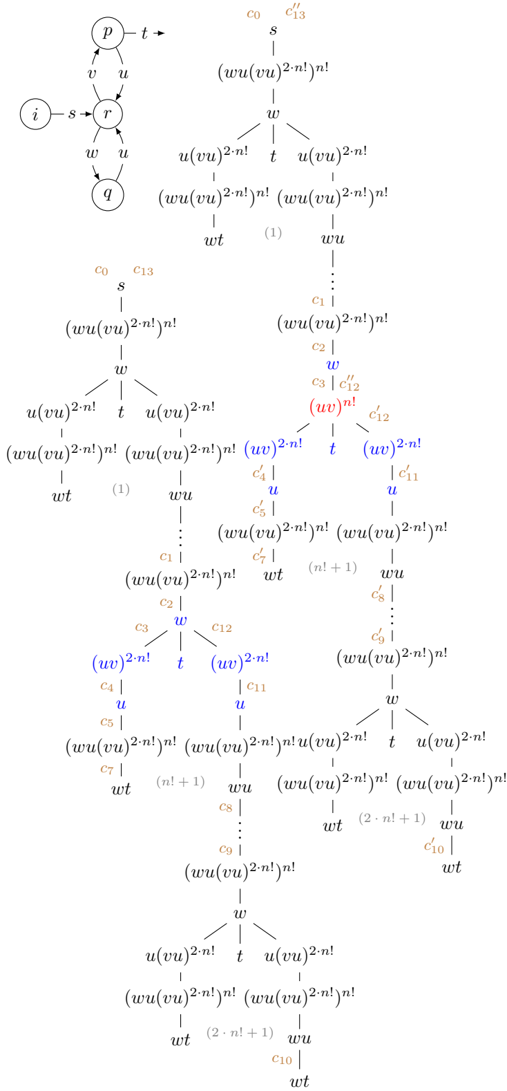
■ Figure 5 Non-HAR gadget and fooling trees in Lemma 29.
