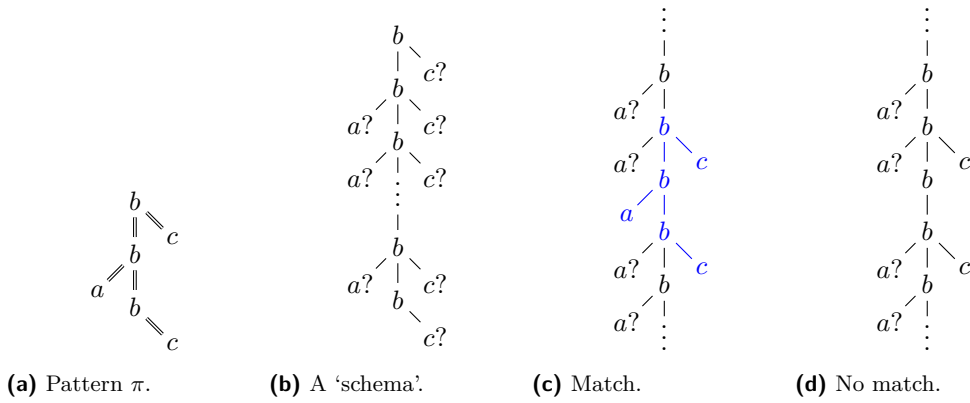
■ Figure 1 Strictly descendent patterns are not stackless.
