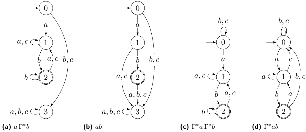
■ Figure 3 Languages of increasing hardness over \Gamma = \{a, b, c\} .
