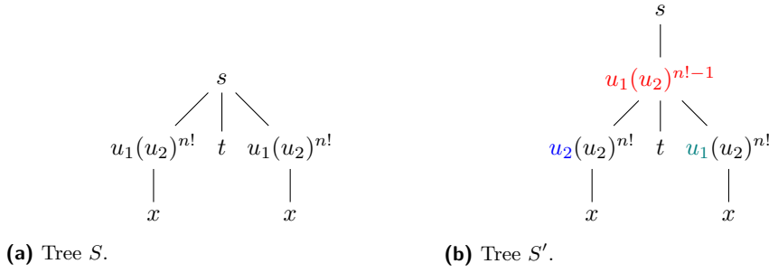
■ Figure 7 Blind variants of fooling trees in Lemma 25.
