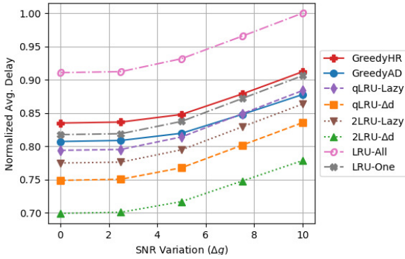
Fig. 5: Heterogeneous SNRs: Berlin topology with density 9.4, g_0 = 10.0\text{dB} , and d_B = 100.0\text{ms} with Akamai trace.
