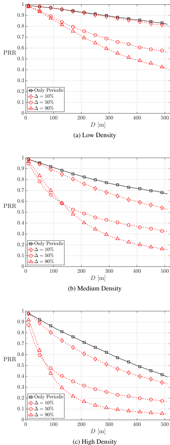
FIGURE 4. PRR as a function of the transmitter-receiver distance D , X = 1000 bytes
