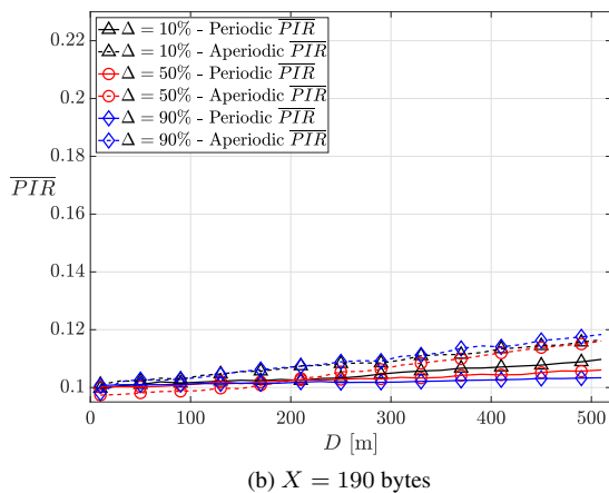
FIGURE 12. Average PIR of aperiodic and periodic traffic as a function of D
