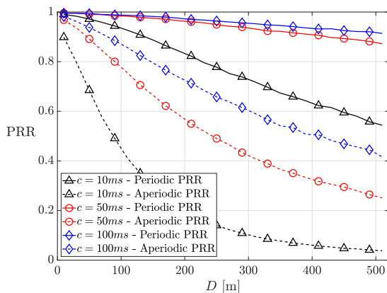
FIGURE 7. PRR for different aperiodic traffic models
