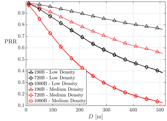
FIGURE 11. PRR when \Delta = 100\%
