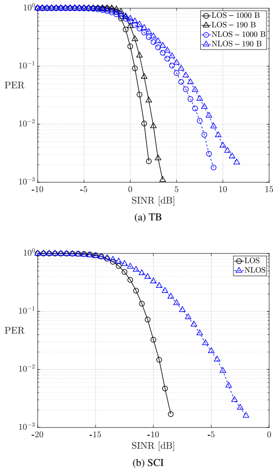
FIGURE 3. PER as a function of average SINR
