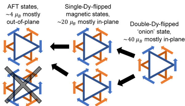
Figure 11. When a strong field is gradually decreased and the order of level crossings enables sequential one-flip transitions (black arrows), the AFT state which is two Dy-flips from the onion state becomes preferentially populated over the FT states (three Dy-flips from the onion state, not shown) and the other AFT state which is four Dy-flips from the onion state.
