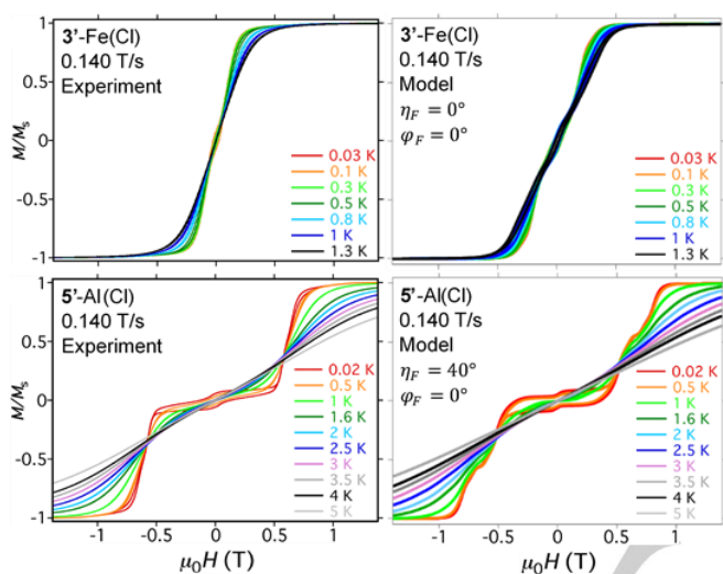
Figure 9. Variable-temperature hysteresis experiments (left) and models (right) for 3' (top) and 5' (bottom). As the temperature is increased, the preference is diminished for spin-phonon relaxation to populate the strongly magnetic onion states at high fields. Thus, saturation is either achieved at stronger fields than for lower temperatures (top), or not at all (bottom). To our knowledge, these are the first variable-temperature hysteresis simulations ever to be reported for lanthanide-based SMMs/SMTs.
