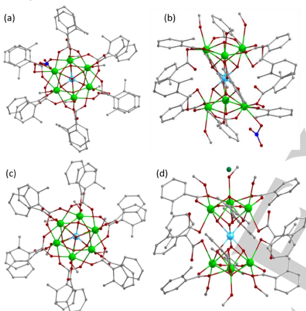
Figure 1. (a) Top and (b) side views of Mn- 2 , showing staggered \{\text{Dy}_3\} rings. Dy atoms green, Mn blue, O red, N blue. NB The disordered MeOH/ \text{NO}_3^- at Dy1 is shown as \text{NO}_3 . (c) Top and (d) side views of Mn- 2' ; Cl in deep green.
