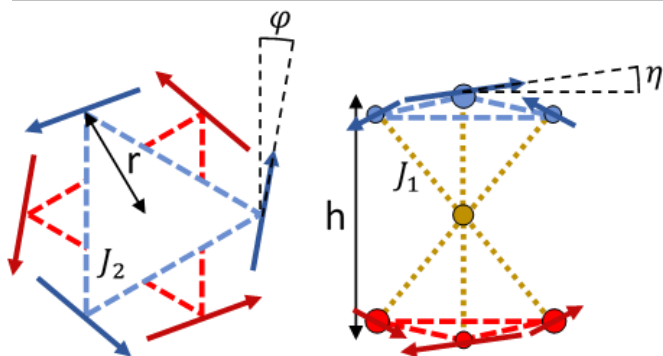
Figure 3. Top-view (left) and side-view (right) schematics of \{Dy_3M^{III}Dy_3\} , showing quantities in Table 1: h = centroid-to-centroid distance, r = average centroid-to-vertex distance, \eta = average out-of-plane angle of Dy easy axes (blue/red arrows), \varphi = average in-plane angle of axes from tangential directions, J_1 = M-Dy exchange coupling constant (dotted yellow lines), J_2 = intra-triangle Dy-Dy exchange coupling constant (dashed blue/red lines). (See SI for Hamiltonians and details of density functional theory (DFT) calculations for J_1 and J_2 .)
