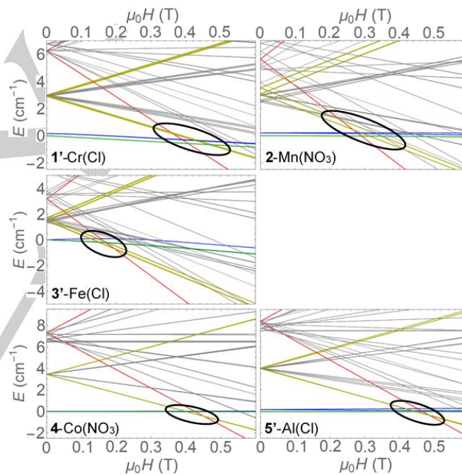
Figure 10. Zeeman spectra for various complexes (see also Fig. S23); external fields oriented in-plane and tangential to {Dy 3 } triangles ( \eta_F = \varphi_F = 0^\circ ). Key level crossings are indicated by black ovals. For clarity, only ground M-eigenstates are shown for each collective Dy state. In order of increasing field-dependence, important Dy states are colour-coded: FT (green); AFT (blue); single-Dy-flipped (yellow); double-Dy-flipped (red). Unimportant Dy-flipped states (not aligned with field) are shown in grey. NB Spectrum for 4 used S_6 -symmetric Dy axes with \eta = 14^\circ , \varphi = 0^\circ ; see SI.
