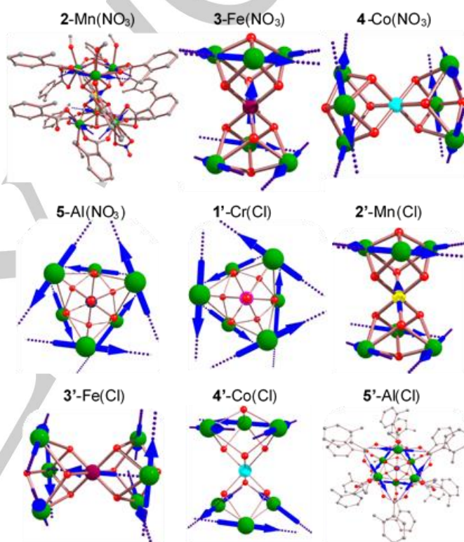
Figure 2. Orientations of magnetic anisotropy axes (dotted lines) in each complex. For illustrative purposes, blue arrows depict the directions of local magnetic moments in one of the ground doublets, being FT for 1'/2'/3'/4'/5'/5' (con-rotatory arrows), and AFT for 2'/3' (counter-rotatory arrows).
