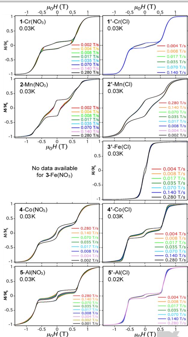
Figure 7. Single-crystal normalised magnetisation ( M/M_S ) vs. applied field for the nitrates (left) and chlorides (right), measured at the temperatures and scan rates indicated. Data for 1 is from Ref. 18.
