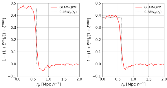
Figure 8. Ratio of the w_{cp,i} -corrected projected correlation function to the true projected correlation function, presented in the form 1 - (1 + \xi^{cp}) / (1 + \xi^{true}) , as obtained in 379 GLAM-QPM mocks and in the model of Hahn et al. (2017) (left: NGC, right: SGC). See the text for details, and fig. 8 of Hahn et al. (2017) for comparison.
