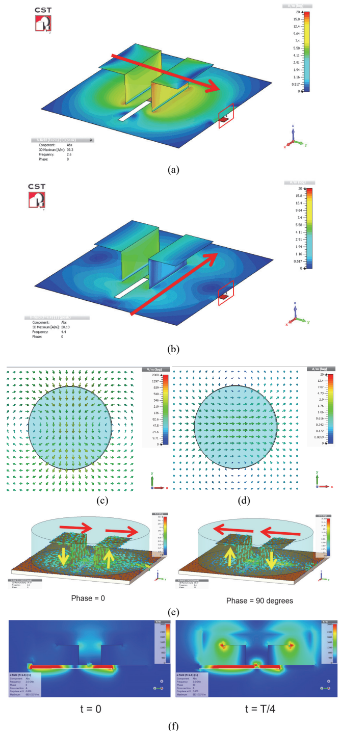
Fig. 7. (a) Simulated surface current distribution at 2.6 GHz. (b) Simulated surface current distribution at 4.4 GHz. (c) Top view of the E-field distribution at 3.1 GHz. (d) Top view of the H-field distribution at 3.1 GHz. (e) Simulated vector current distribution at two different phase angles. The current directions have been marked. (f) Electric-field side views at different periods of time.
