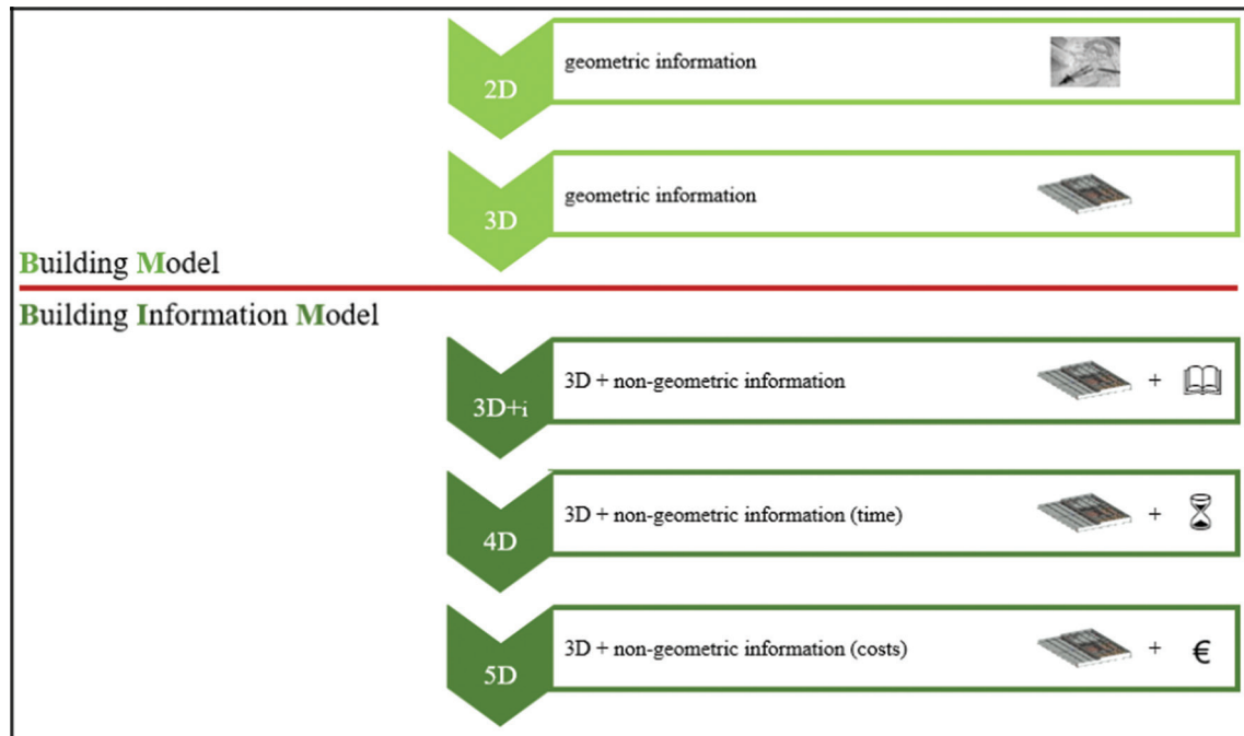
Fig. 3: Building information modelling vs. conventional planning.
