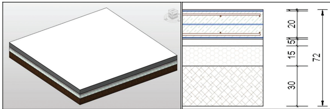
Fig. 5: Module of the floor plate.
