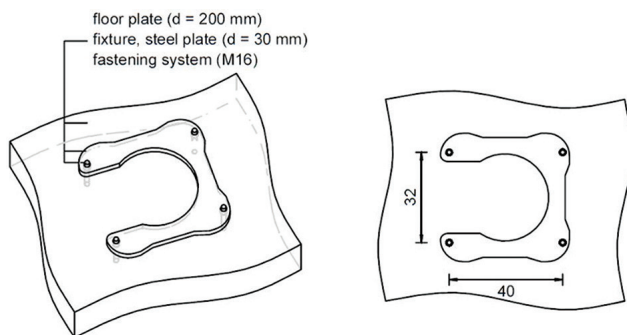
Fig. 6: Fastening system for the fixture of the robotic machine (dimensions in cm unless otherwise noted).
