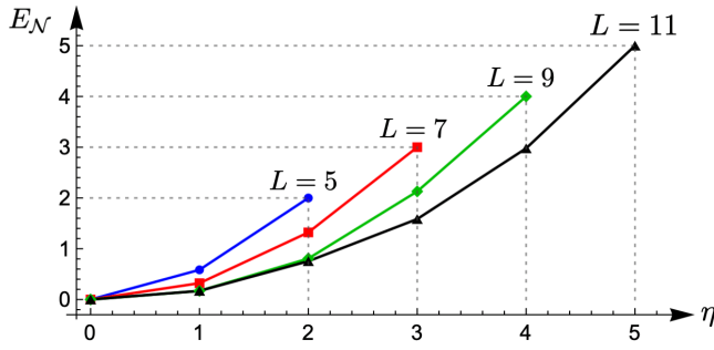
FIG. 2. Log negativity E_N , measuring entanglement between left and right halves, in steady states corresponding to different symmetry sectors \eta and number of sites L , with \gamma_+ = \gamma_- .
