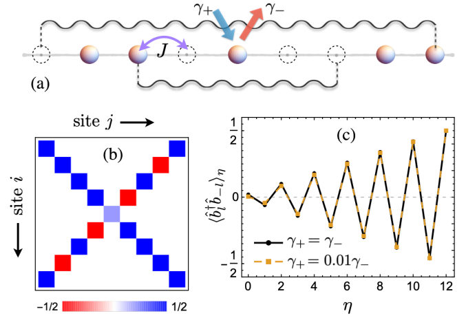
FIG. 1. (a) Schematic setup showing coherent tunneling J and incoherent pump and loss \gamma_{\pm} at the center. The system has a strong dynamical symmetry that stabilizes long-range entangled particle-hole pairs at reflection-symmetric sites. (b) Single-particle density matrix \langle \hat{b}_i^\dagger \hat{b}_j \rangle in the steady state with maximum number of Bell pairs. The center has occupation \gamma_+ / (\gamma_+ + \gamma_-) . (c) End-to-end coherence for different symmetry sectors \eta .
