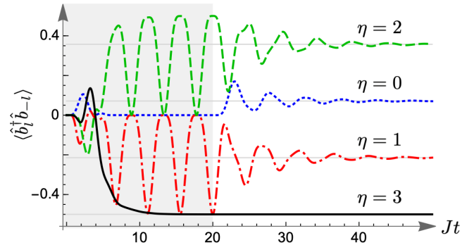
FIG. 3. End-to-end correlation during a selective preparation of different symmetry sectors \eta for L = 7 . The shaded region shows the generation of Bell pairs from symmetric Fock states, \hat{b}_0^\dagger \prod_{k=1}^l \hat{b}_k^\dagger \hat{b}_{-k}^\dagger |0\rangle , driven by the loss of JW fermions at the center with rate \gamma_F = 3J . The white region shows subsequent dynamics with boson pump and loss rates \gamma_\pm = 2J .
