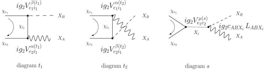
Figure 9: Generic tree-level amplitudes in \chi\chi \rightarrow X_A X_B annihilations, referring to VV , VS and SS -type final state particles X_A X_B . The generic form of s -channel exchange diagrams for X_A X_B = \eta\bar{\eta} final states agrees with the s -channel diagram above. The vertex-factors V_{ei}^{\rho(d)} are defined as V_{ei}^{\rho(d)} = \gamma^\rho (r_{ei}^{(d)} + q_{ei}^{(d)} \gamma_5) , if attached to a three-point vertex with a gauge-boson (with Lorentz-index \rho ), and V_{ei}^{\rho(d)} = (r_{ei}^{(d)} + q_{ei}^{(d)} \gamma_5) , if associated with a vertex that involves a scalar particle X_A , X_B or X_i . Here the expression r_{ei}^{(d)} ( q_{ei}^{(d)} ) either denotes a vector or scalar (an axial-vector or pseudo-scalar) type of coupling factor. For the definition of c_{ABX_i} and the Lorentz structures L_{ABX_i} we refer to Tab. 4 below.
