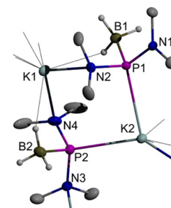
Figure 2. Graphical representation of the crystallographically independent formula units in crystalline K[1 b]. For clarity, hydrogen atoms except those of \text{BH}_3 groups were omitted. Thermal ellipsoids of heavy atoms were drawn at the 50% probability level. Selected distances (in Å): P1–N1 1.697(2), P1–N2 1.741(2), P1–B1 1.947(3), P1–K2 3.301(1), P2–N3 1.736(2), P2–N4 1.725(2), P2–B2 1.935(4), P2–K2 3.352(1), K1–N2 2.849(2), K1–N4 2.932(2), K1–H(B1) 2.86(3), K1–H(B2) 2.72(3), K2–N3#1 2.961(2).
