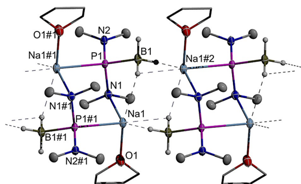
Figure 1. Graphical representation of two dimeric units in crystalline Na(THF)[1 b]. For clarity, hydrogen atoms except those of \text{BH}_3 groups were omitted and carbon atoms in THF ligands represented using a wire model. Thermal ellipsoids of heavy atoms were drawn at the 50% probability level. Selected distances (in Å): P1–N1 1.752(1), P1–N2 1.699(1), P1–B1 1.937(2), P1–Na1#1 2.963(1), Na1–O1 2.311(1), Na1–N1 2.520(1), B1–Na1#2 2.682(2), B1–Na1 3.361(2).
