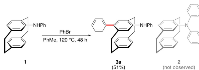
Scheme 2. Pd-catalyzed para -selective C–H activation/aryl–aryl coupling under classical Buchwald–Hartwig- amination of N -phenylamino[2.2]paracyclophane (0.5 mmol, 0.17 M): PhBr (0.6 mmol), Pd 2 dba 3 (5.0 mol%), SPhos (5.0 mol%), KO t Bu (1.0 mmol), PhMe, 120 °C, 48 h.
