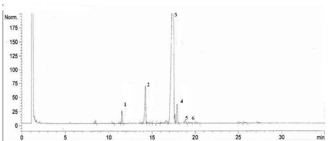
Fig. 1. Gas chromatogram of the sterols fraction from Evening Primrose Oil. 1. \alpha -Colesterol.
