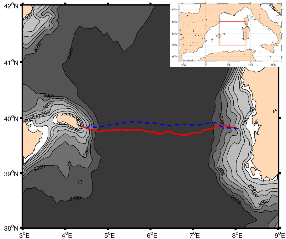
Fig. 1. Path of the glider overimpressed on the bathymetry of the Balearic Sea area. Outward (red) and return (blue) trips are represented.
