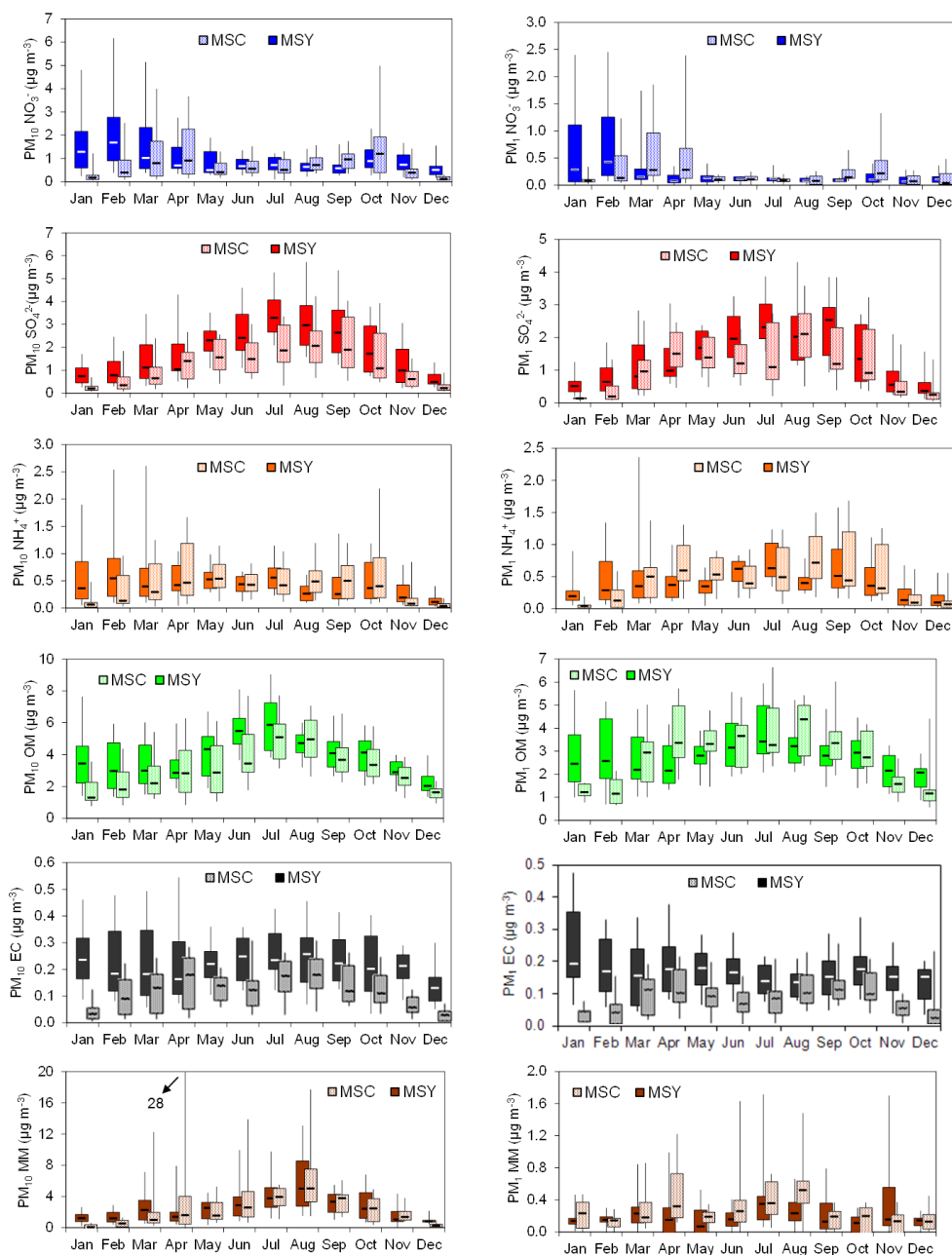
Figure 6. Monthly median (black line within the boxes) and percentiles (5–25–75–95, boxes and whiskers) of major PM_{10} and PM_1 chemical components concentrations at Montsec (MSC) and Montseny (MSY) based on daily measurements between January 2010 and March 2013.
