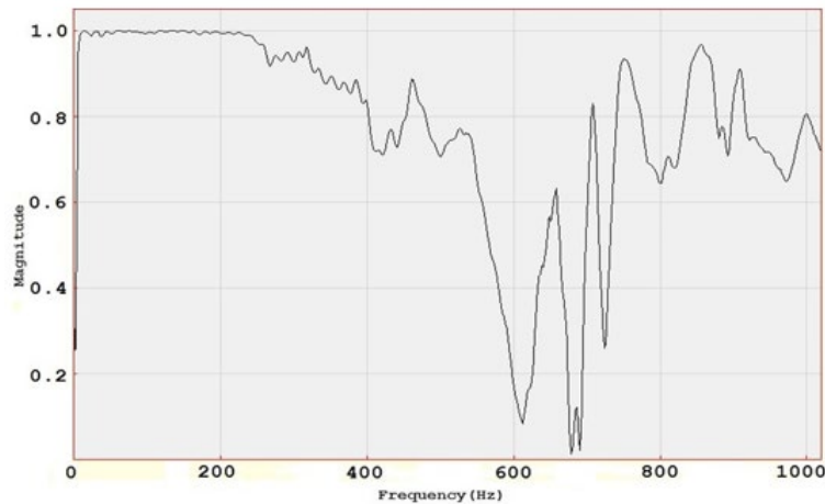
Figure 9. The coherence of measurement when using one accelerometer.
