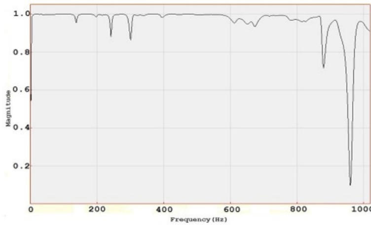
Figure 10. The coherence of measurement when using three accelerometers.
