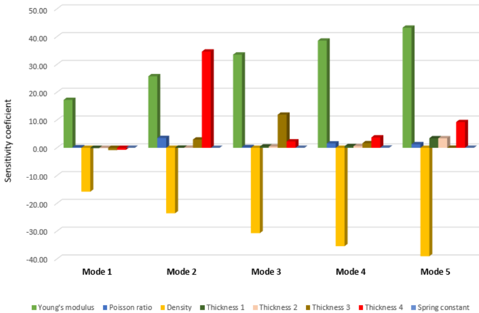
Figure 13. Sensitivity coefficients for potential updating parameters of BIW model with CELAS elements.
