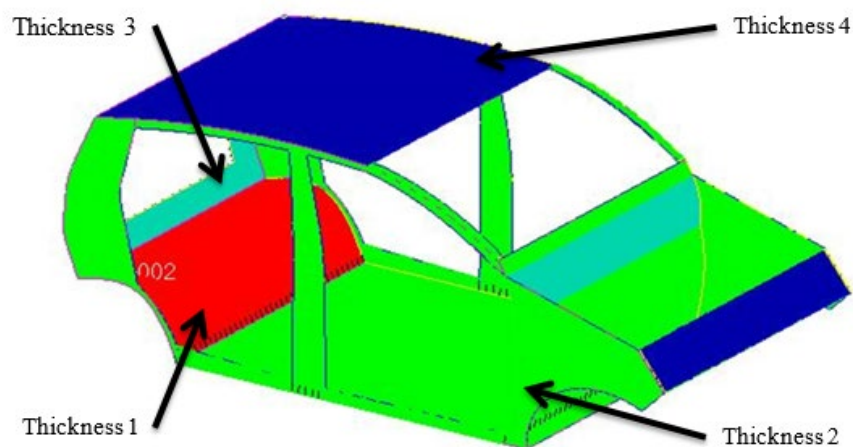
Figure 1. The assignment of different thickness on the BIW model
