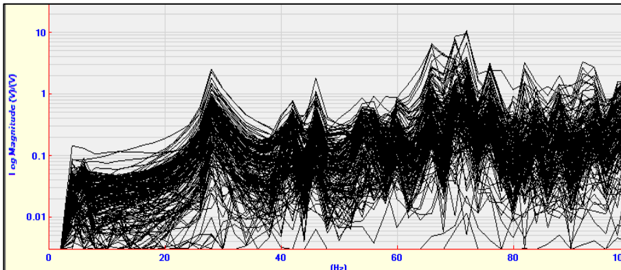
Figure 7. Response sample of roving accelerometer impact hammer test with three accelerometers.
