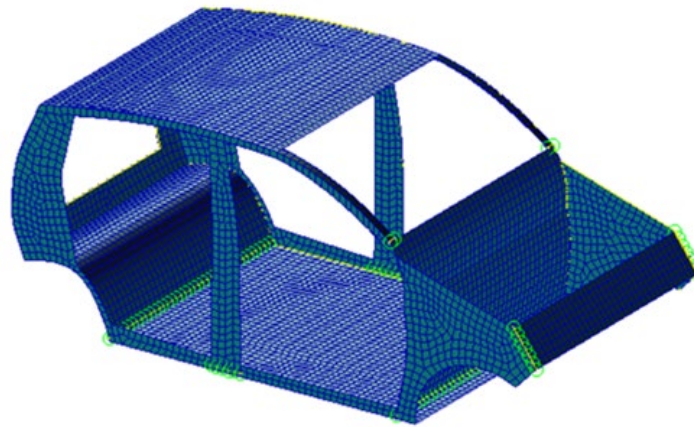
Figure 2. Locations of the joint element that are created on the BIW model.
