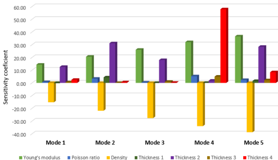
Figure 11. Sensitivity coefficient for potential updating parameters of BIW model without joint elements.
