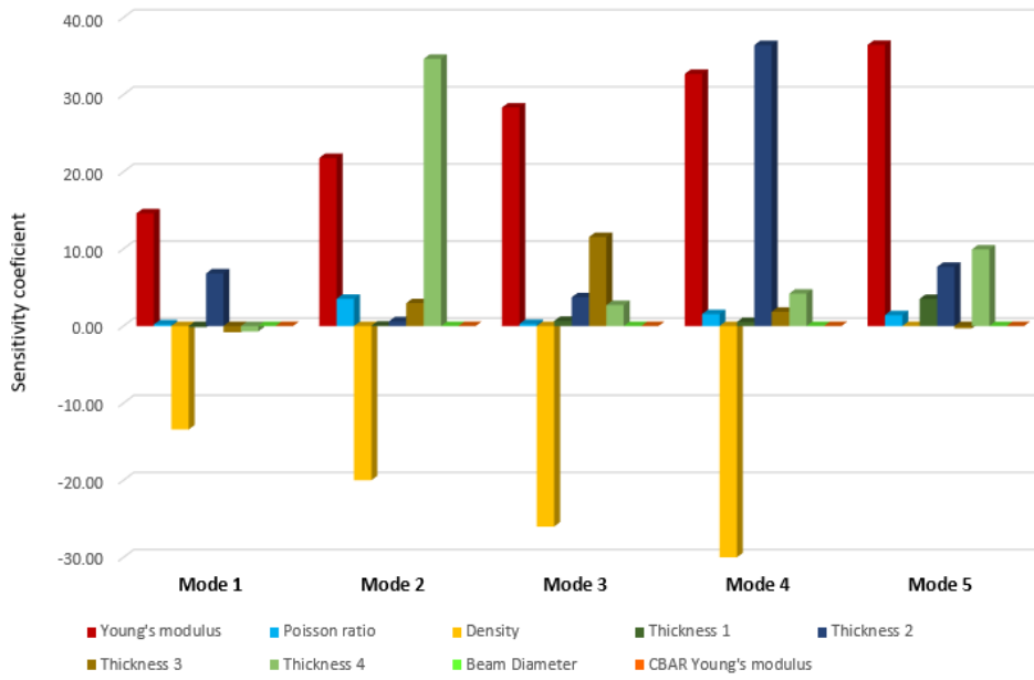
Figure 12. Sensitivity coefficients for potential updating parameters of BIW model with CBAR elements.
