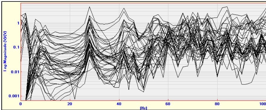
Figure 6. Response sample of roving hammer impact hammer test with one accelerometer.
