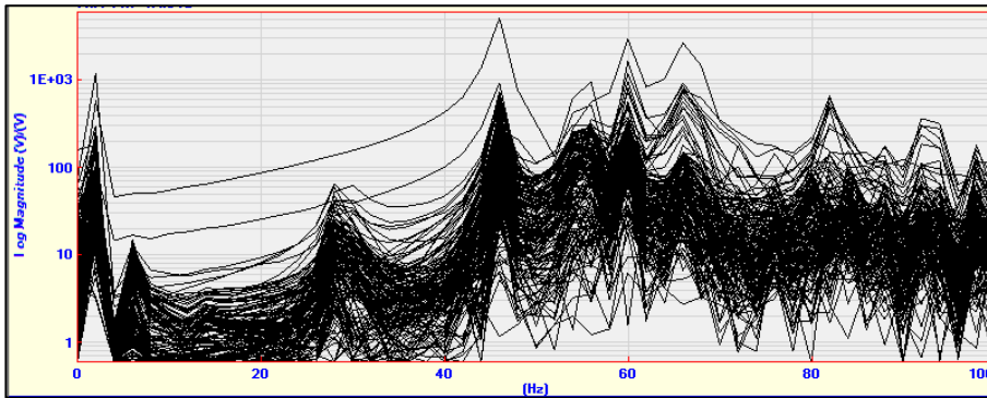
Figure 5. Response sample of roving accelerometer impact hammer with one accelerometer.
